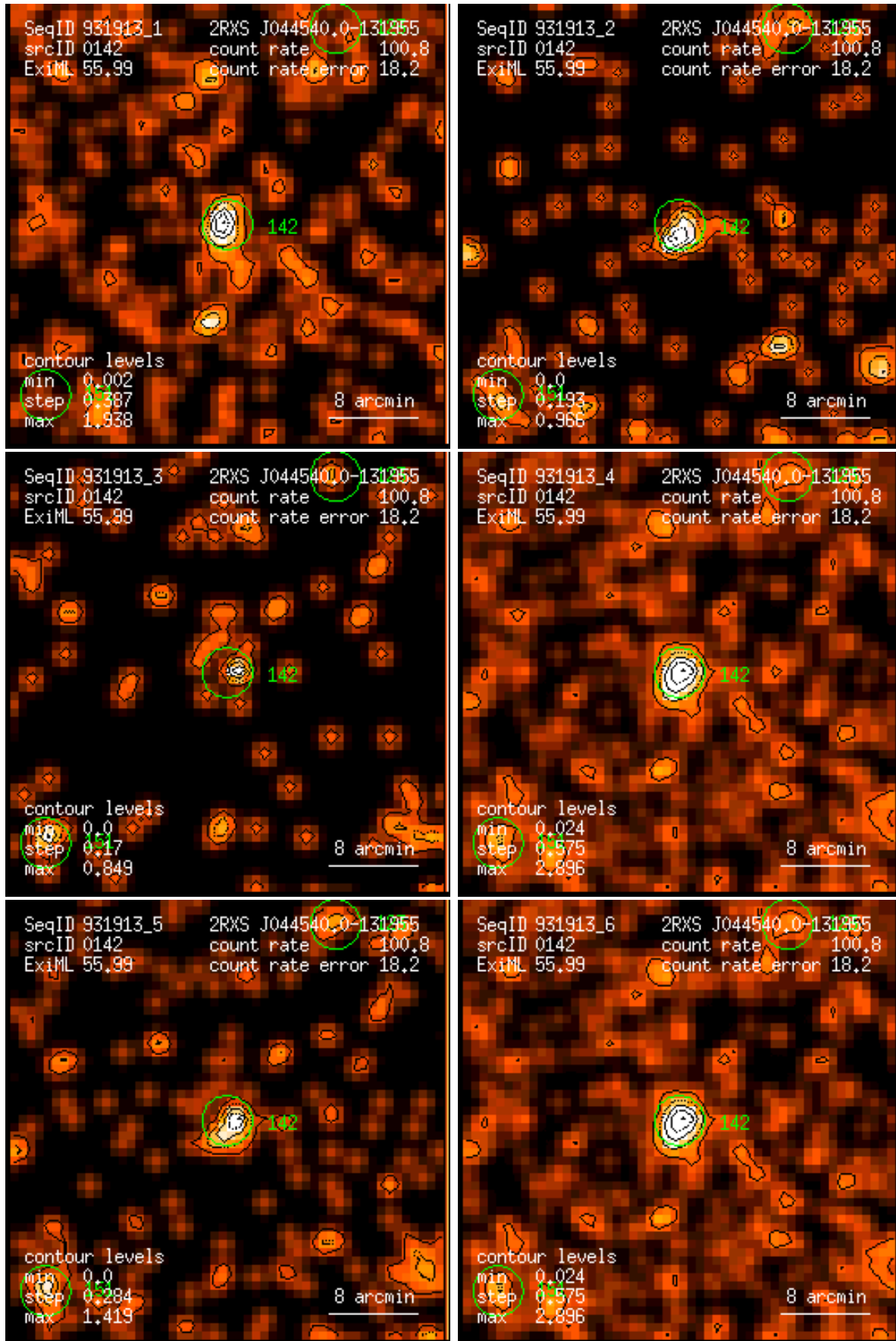
Figure 142: RASS 931913: detection 0142: band rate images, Gaussian filter: (1) PSPC channels 11 – 41, (2) 52 – 90, (3) 91 – 201, (4) 11 – 235, (5) 52 – 201, (6) 11 – 201. Broad band rates in counts/ks. Band rate contour levels in counts/ks/arcmin 2 .
