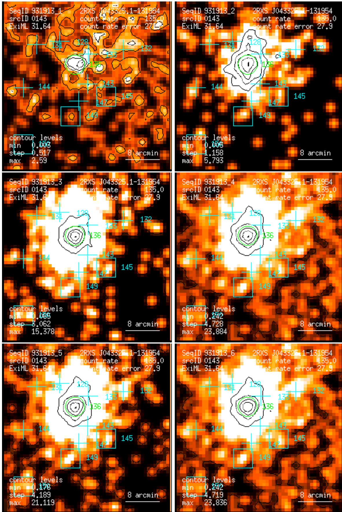
Figure 143: RASS 931913: detection 0143: band rate images, Gaussian filter: (1) PSPC channels 11 – 41, (2) 52 – 90, (3) 91 – 201, (4) 11 – 235, (5) 52 – 201, (6) 11 – 201. Broad band rates in counts/ks. Band rate contour levels in counts/ks/arcmin 2 .
