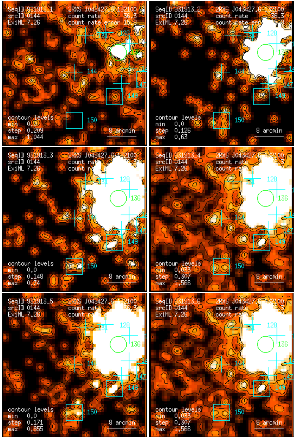
Figure 144: RASS 931913: detection 0144: band rate images, Gaussian filter: (1) PSPC channels 11 – 41, (2) 52 – 90, (3) 91 – 201, (4) 11 – 235, (5) 52 – 201, (6) 11 – 201. Broad band rates in counts/ks. Band rate contour levels in counts/ks/arcmin 2 .
