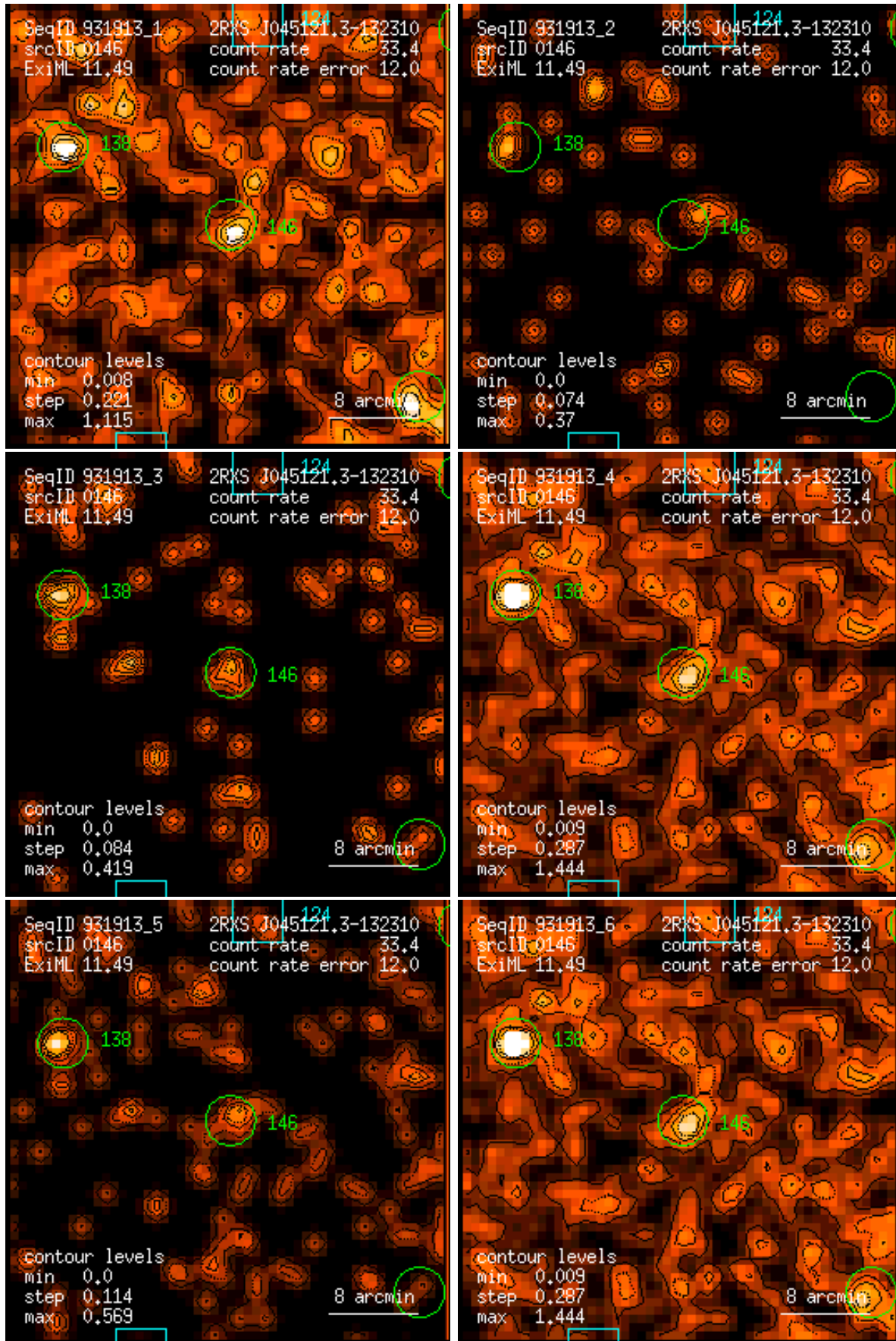
Figure 146: RASS 931913: detection 0146: band rate images, Gaussian filter: (1) PSPC channels 11 – 41, (2) 52 – 90, (3) 91 – 201, (4) 11 – 235, (5) 52 – 201, (6) 11 – 201. Broad band rates in counts/ks. Band rate contour levels in counts/ks/arcmin 2 .
