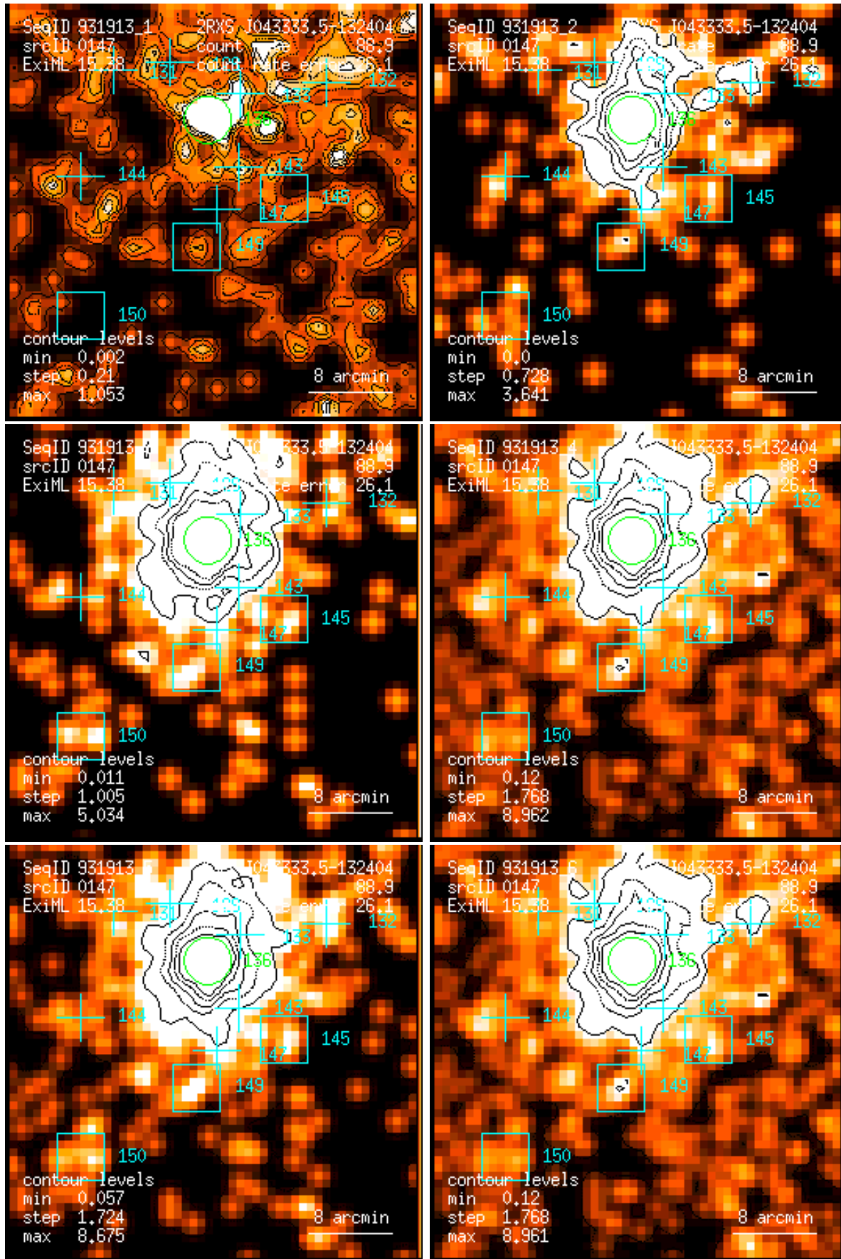
Figure 147: RASS 931913: detection 0147: band rate images, Gaussian filter: (1) PSPC channels 11 – 41, (2) 52 – 90, (3) 91 – 201, (4) 11 – 235, (5) 52 – 201, (6) 11 – 201. Broad band rates in counts/ks. Band rate contour levels in counts/ks/arcmin 2 .
