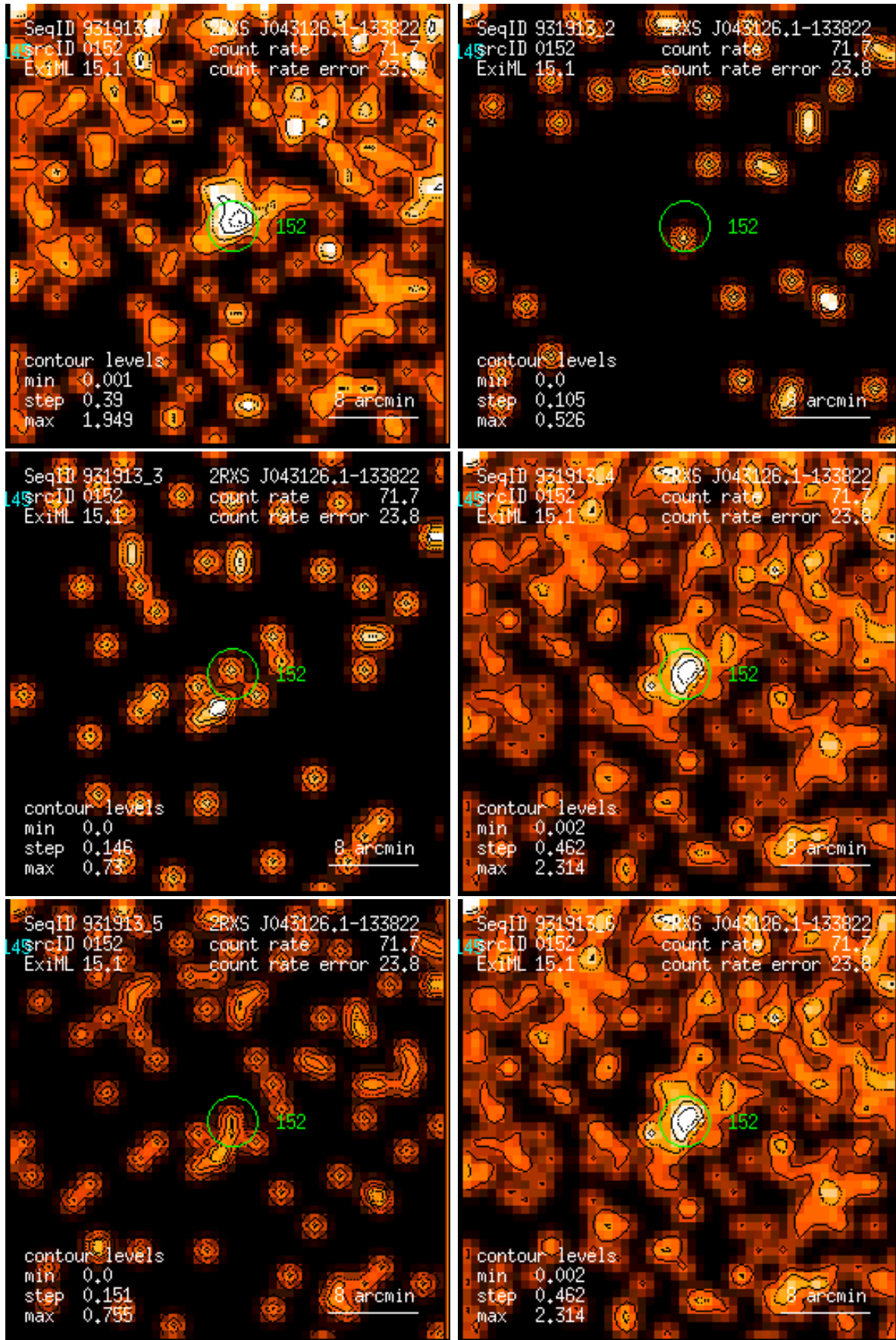
Figure 152: RASS 931913: detection 0152: band rate images, Gaussian filter: (1) PSPC channels 11 – 41, (2) 52 – 90, (3) 91 – 201, (4) 11 – 235, (5) 52 – 201, (6) 11 – 201. Broad band rates in counts/ks. Band rate contour levels in counts/ks/arcmin 2 .
