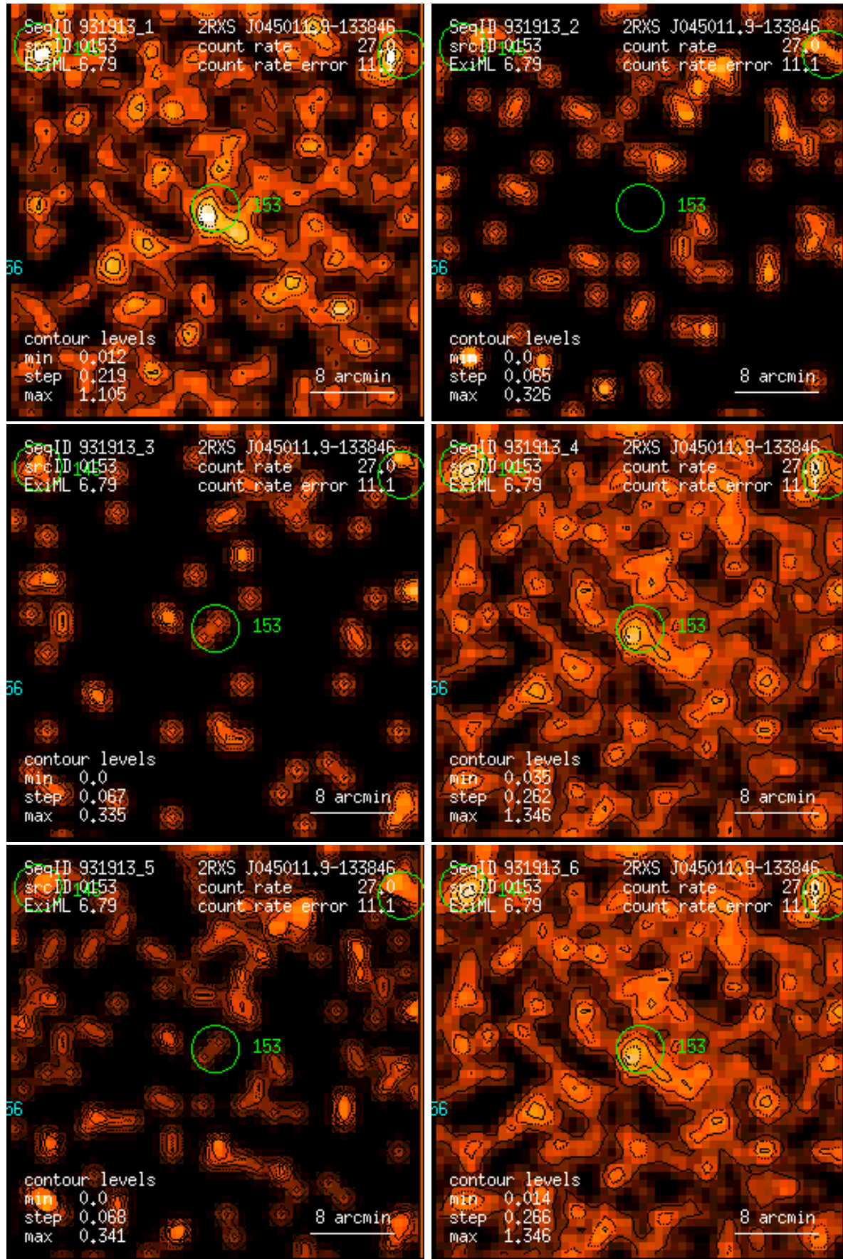
Figure 153: RASS 931913: detection 0153: band rate images, Gaussian filter: (1) PSPC channels 11 – 41, (2) 52 – 90, (3) 91 – 201, (4) 11 – 235, (5) 52 – 201, (6) 11 – 201. Broad band rates in counts/ks. Band rate contour levels in counts/ks/arcmin 2 .
