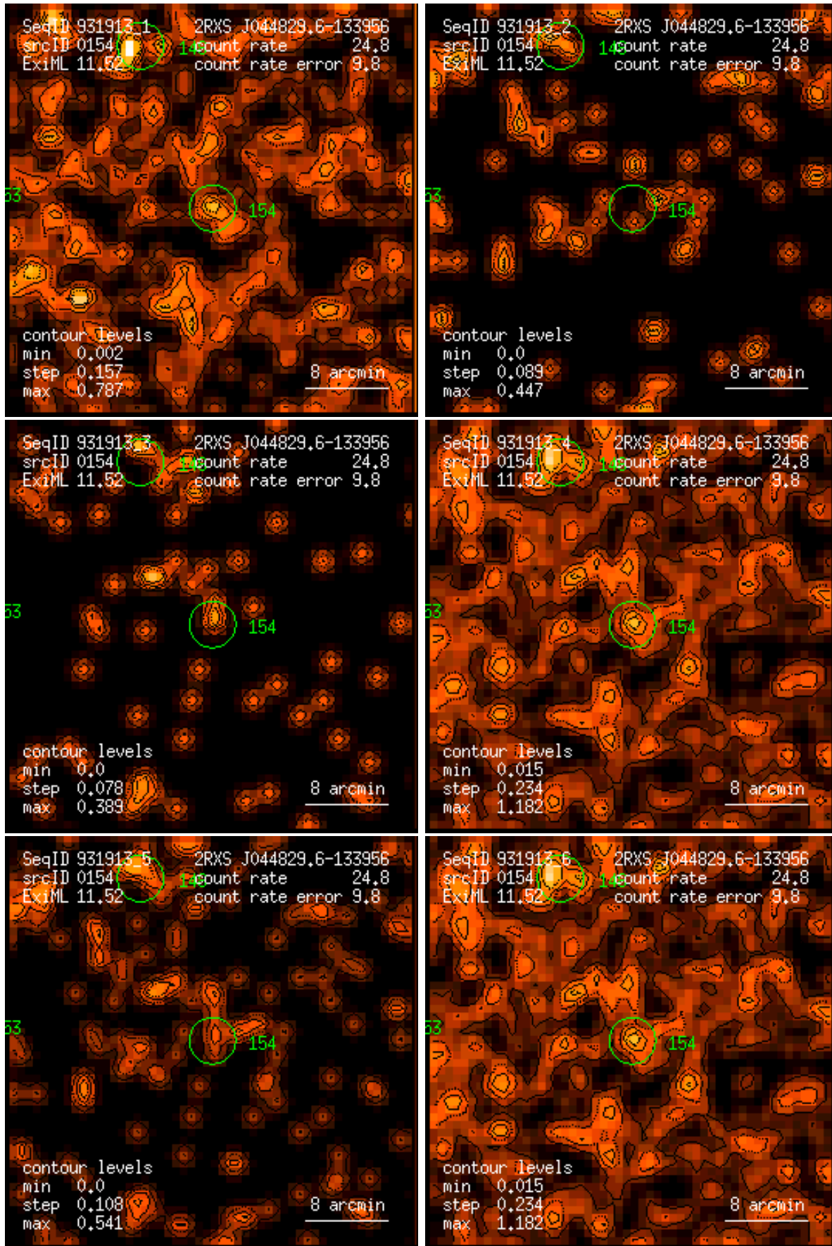
Figure 154: RASS 931913: detection 0154: band rate images, Gaussian filter: (1) PSPC channels 11 – 41, (2) 52 – 90, (3) 91 – 201, (4) 11 – 235, (5) 52 – 201, (6) 11 – 201. Broad band rates in counts/ks. Band rate contour levels in counts/ks/arcmin 2 .
