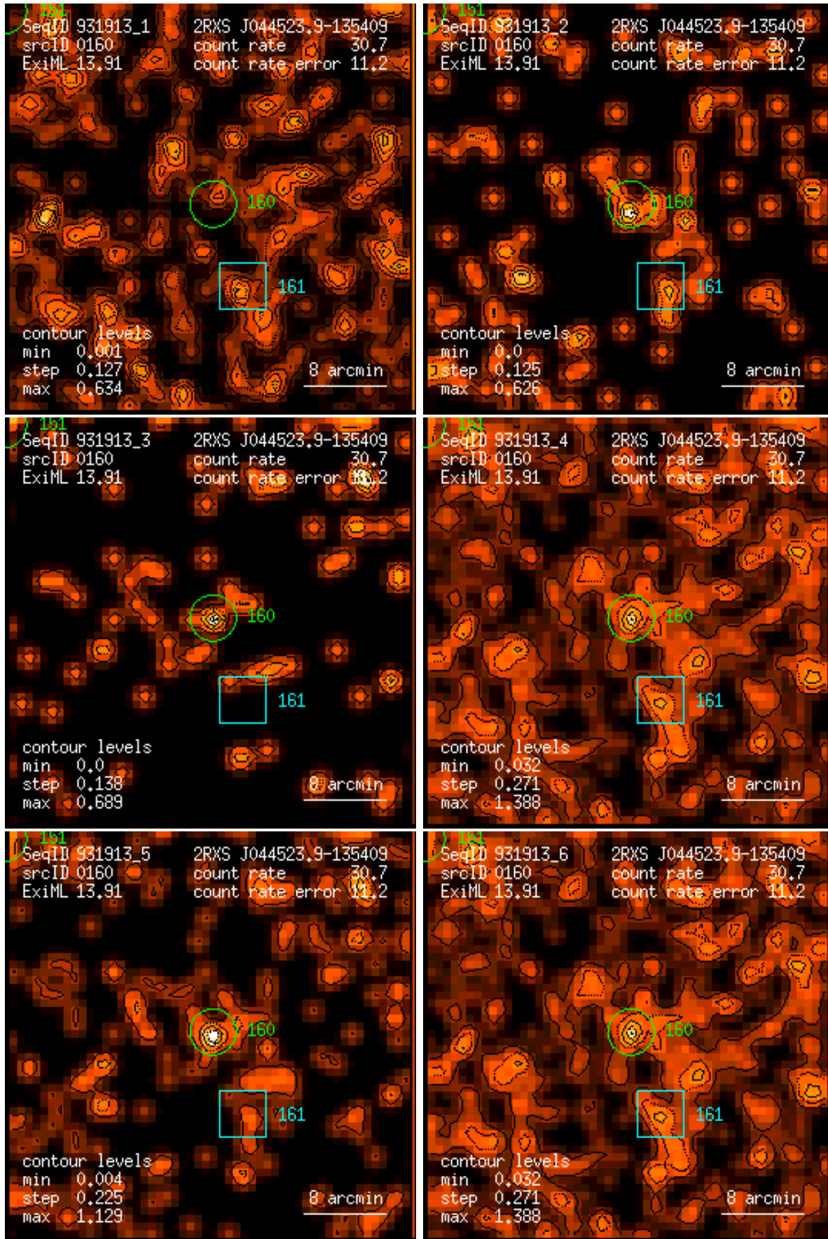
Figure 160: RASS 931913: detection 0160: band rate images, Gaussian filter: (1) PSPC channels 11 – 41, (2) 52 – 90, (3) 91 – 201, (4) 11 – 235, (5) 52 – 201, (6) 11 – 201. Broad band rates in counts/ks. Band rate contour levels in counts/ks/arcmin 2 .
