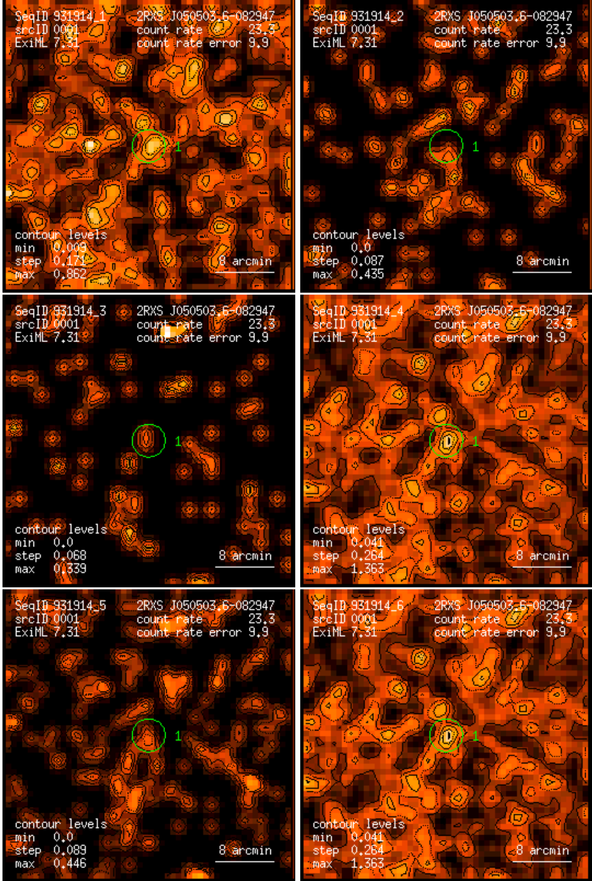
Figure 1: RASS 931914: detection 0001: band rate images, Gaussian filter: (1) PSPC channels 11 – 41, (2) 52 – 90, (3) 91 – 201, (4) 11 – 235, (5) 52 – 201, (6) 11 – 201. Broad band rates in counts/ks. Band rate contour levels in counts/ks/arcmin 2 .
