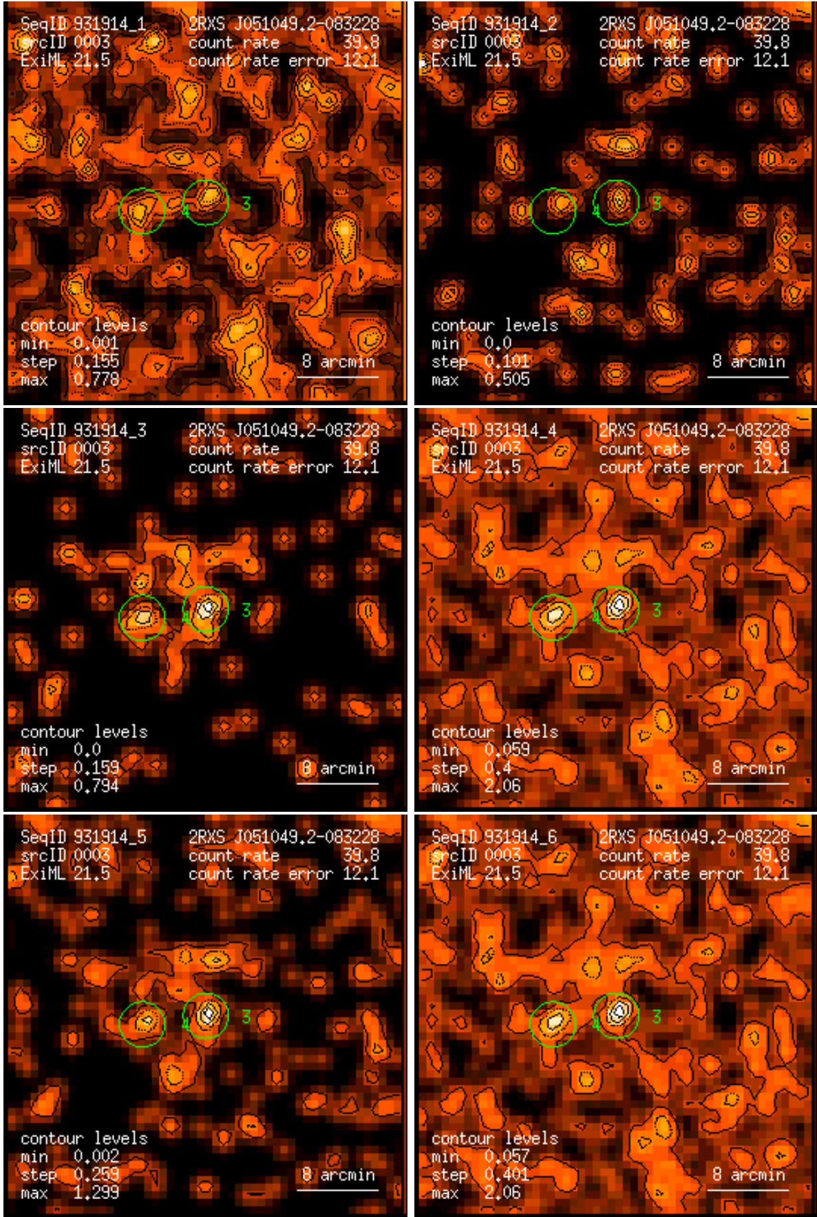
Figure 3: RASS 931914: detection 0003: band rate images, Gaussian filter: (1) PSPC channels 11 – 41, (2) 52 – 90, (3) 91 – 201, (4) 11 – 235, (5) 52 – 201, (6) 11 – 201. Broad band rates in counts/ks. Band rate contour levels in counts/ks/arcmin 2 .
