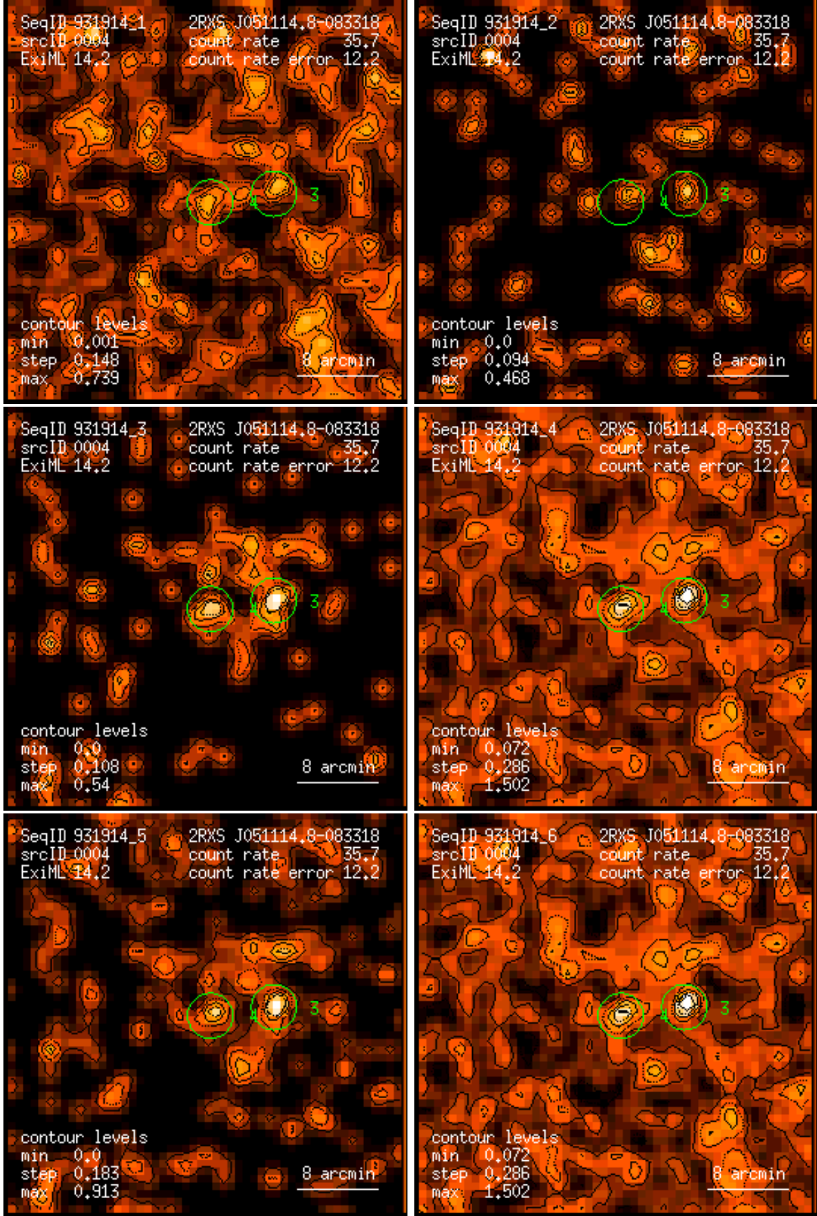
Figure 4: RASS 931914: detection 0004: band rate images, Gaussian filter: (1) PSPC channels 11 – 41, (2) 52 – 90, (3) 91 – 201, (4) 11 – 235, (5) 52 – 201, (6) 11 – 201. Broad band rates in counts/ks. Band rate contour levels in counts/ks/arcmin 2 .
