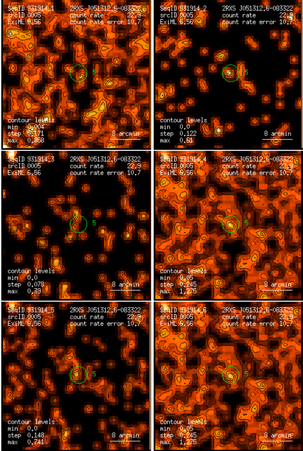
Figure 5: RASS 931914: detection 0005: band rate images, Gaussian filter: (1) PSPC channels 11 – 41, (2) 52 – 90, (3) 91 – 201, (4) 11 – 235, (5) 52 – 201, (6) 11 – 201. Broad band rates in counts/ks. Band rate contour levels in counts/ks/arcmin 2 .
