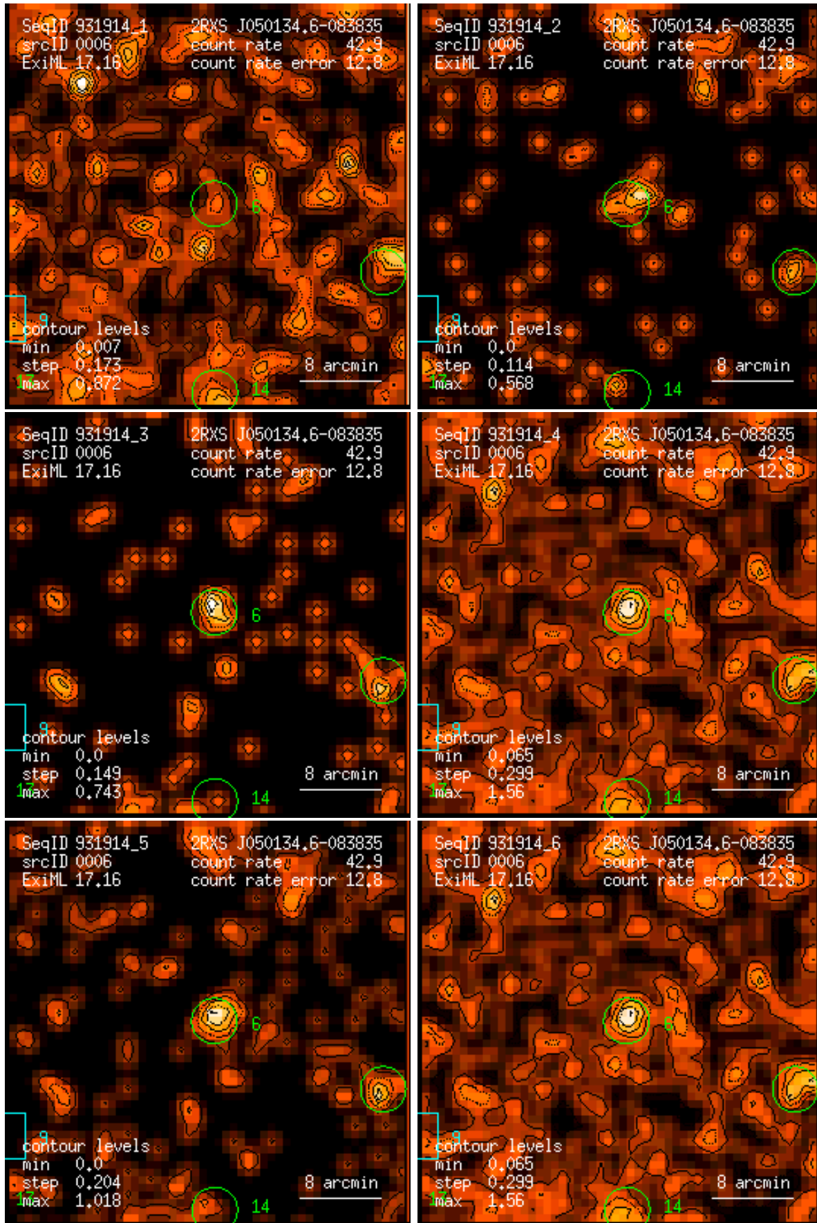
Figure 6: RASS 931914: detection 0006: band rate images, Gaussian filter: (1) PSPC channels 11 – 41, (2) 52 – 90, (3) 91 – 201, (4) 11 – 235, (5) 52 – 201, (6) 11 – 201. Broad band rates in counts/ks. Band rate contour levels in counts/ks/arcmin 2 .
