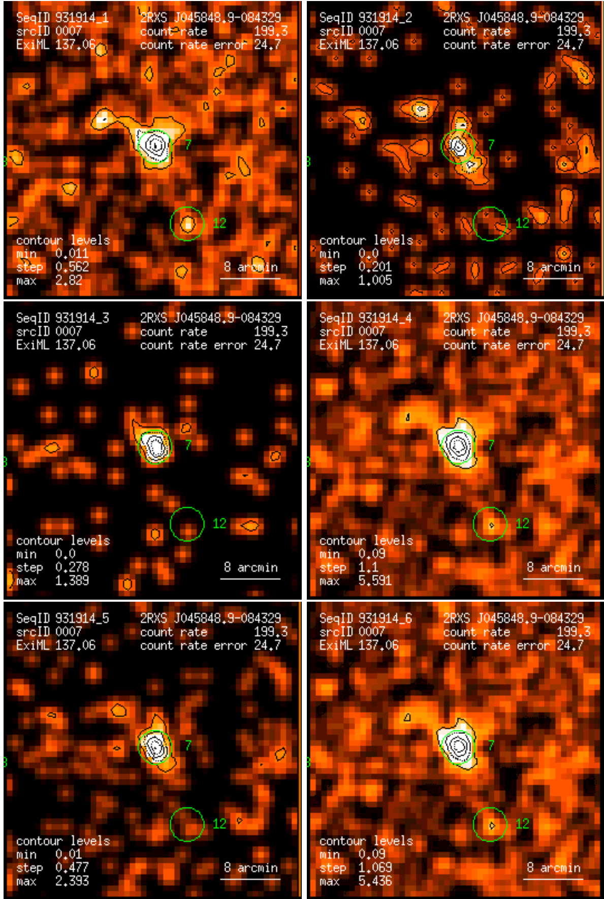
Figure 7: RASS 931914: detection 0007: band rate images, Gaussian filter: (1) PSPC channels 11 – 41, (2) 52 – 90, (3) 91 – 201, (4) 11 – 235, (5) 52 – 201, (6) 11 – 201. Broad band rates in counts/ks. Band rate contour levels in counts/ks/arcmin 2 .
