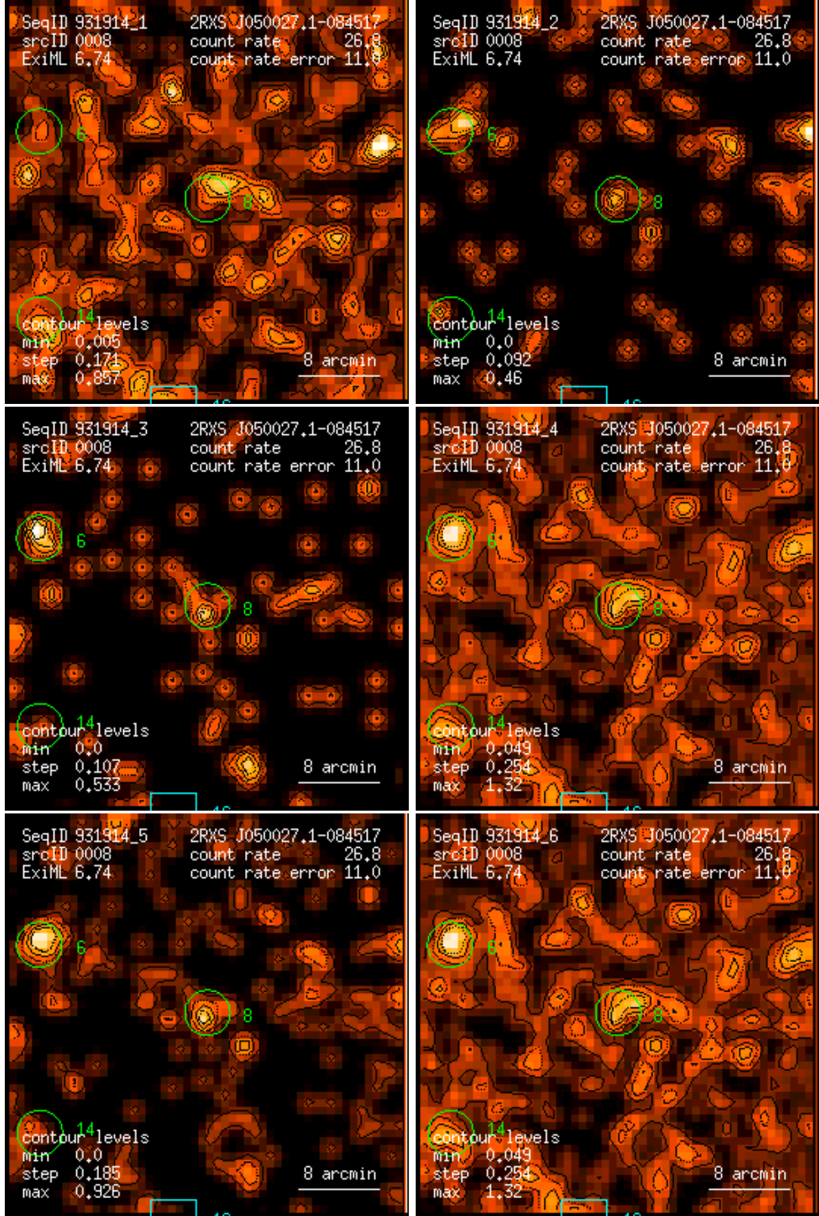
Figure 8: RASS 931914: detection 0008: band rate images, Gaussian filter: (1) PSPC channels 11 – 41, (2) 52 – 90, (3) 91 – 201, (4) 11 – 235, (5) 52 – 201, (6) 11 – 201. Broad band rates in counts/ks. Band rate contour levels in counts/ks/arcmin 2 .
