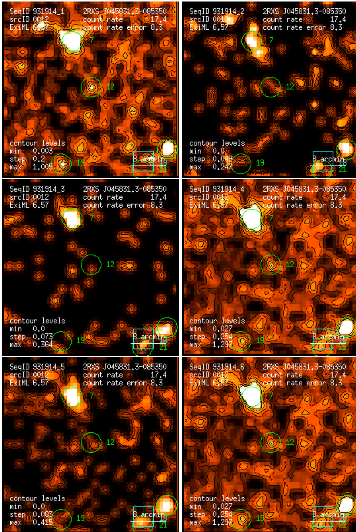
Figure 12: RASS 931914: detection 0012: band rate images, Gaussian filter: (1) PSPC channels 11 – 41, (2) 52 – 90, (3) 91 – 201, (4) 11 – 235, (5) 52 – 201, (6) 11 – 201. Broad band rates in counts/ks. Band rate contour levels in counts/ks/arcmin 2 .
