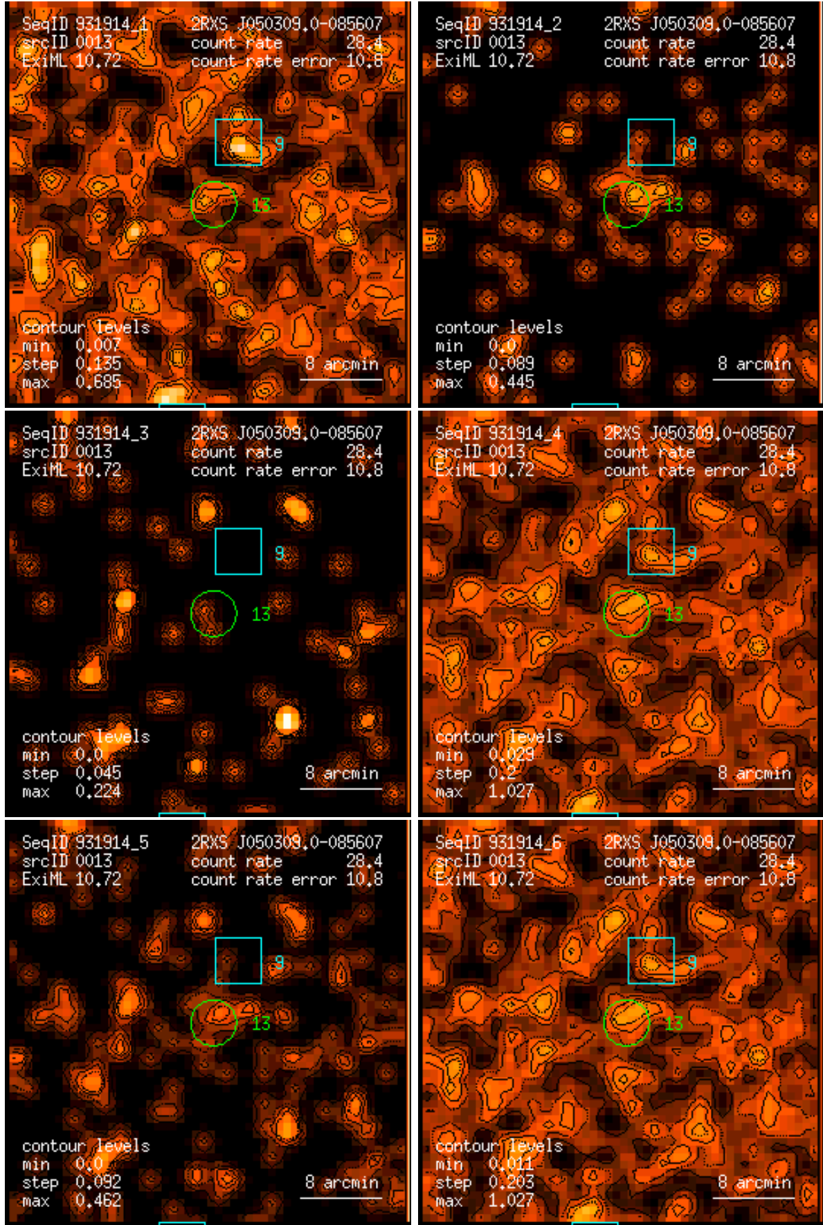
Figure 13: RASS 931914: detection 0013: band rate images, Gaussian filter: (1) PSPC channels 11 – 41, (2) 52 – 90, (3) 91 – 201, (4) 11 – 235, (5) 52 – 201, (6) 11 – 201. Broad band rates in counts/ks. Band rate contour levels in counts/ks/arcmin 2 .
