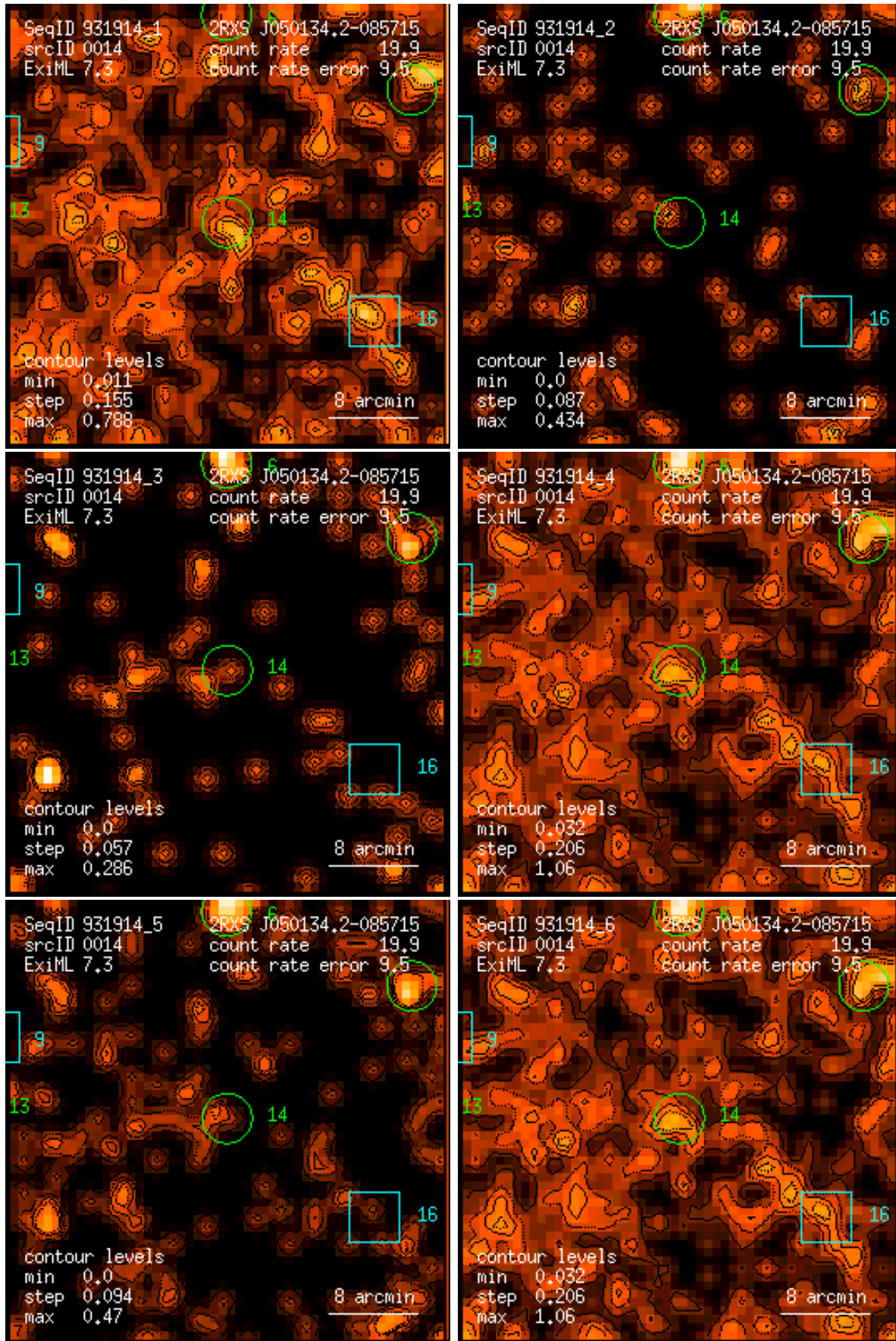
Figure 14: RASS 931914: detection 0014: band rate images, Gaussian filter: (1) PSPC channels 11 – 41, (2) 52 – 90, (3) 91 – 201, (4) 11 – 235, (5) 52 – 201, (6) 11 – 201. Broad band rates in counts/ks. Band rate contour levels in counts/ks/arcmin 2 .
