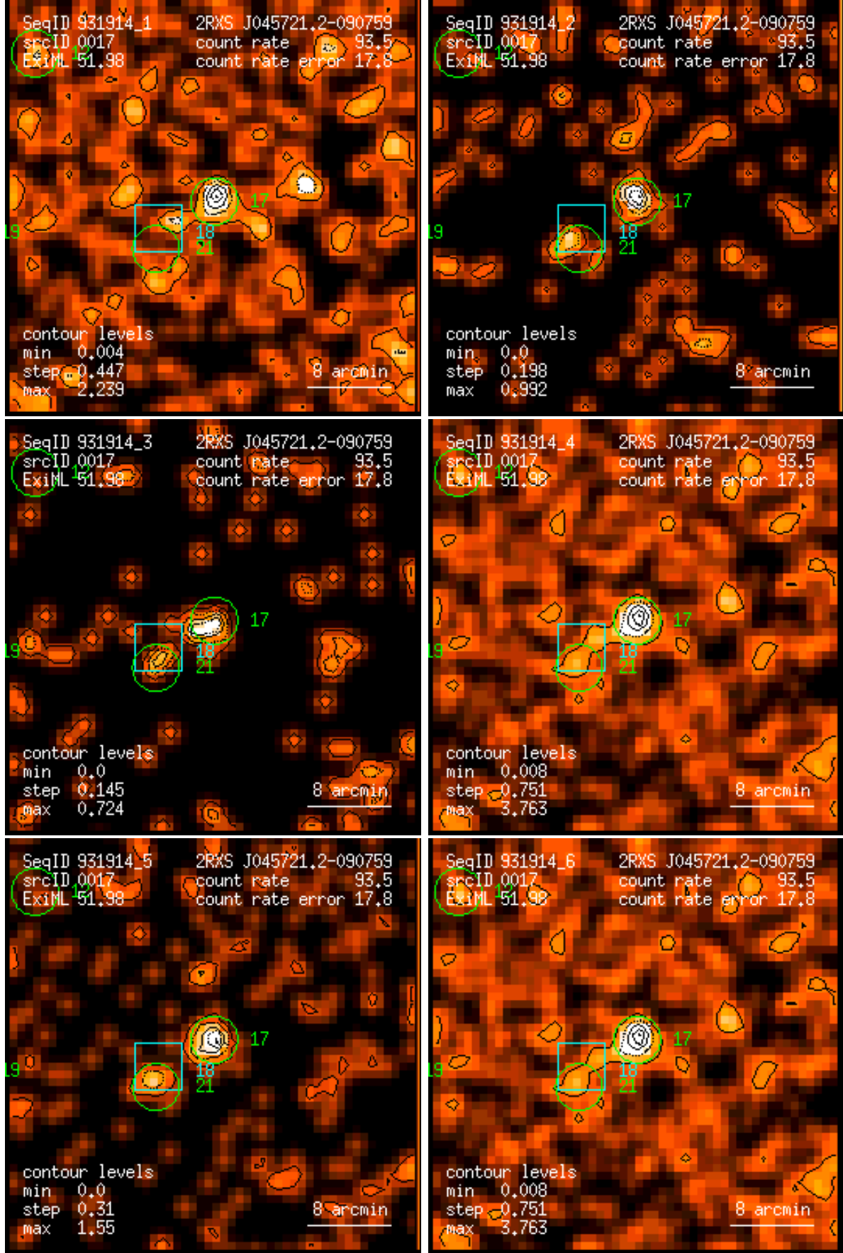
Figure 17: RASS 931914: detection 0017: band rate images, Gaussian filter: (1) PSPC channels 11 – 41, (2) 52 – 90, (3) 91 – 201, (4) 11 – 235, (5) 52 – 201, (6) 11 – 201. Broad band rates in counts/ks. Band rate contour levels in counts/ks/arcmin 2 .
