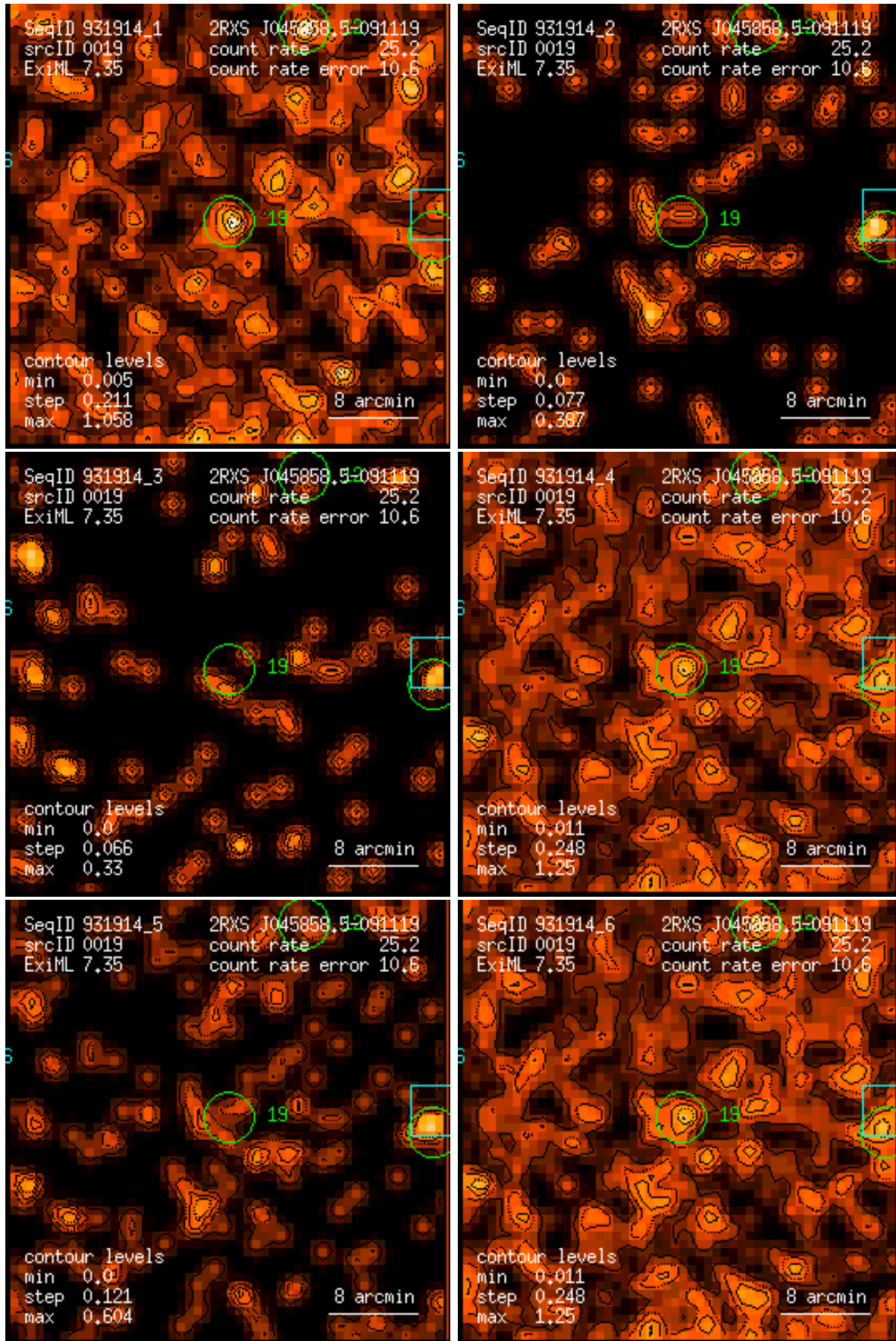
Figure 19: RASS 931914: detection 0019: band rate images, Gaussian filter: (1) PSPC channels 11 – 41, (2) 52 – 90, (3) 91 – 201, (4) 11 – 235, (5) 52 – 201, (6) 11 – 201. Broad band rates in counts/ks. Band rate contour levels in counts/ks/arcmin 2 .
