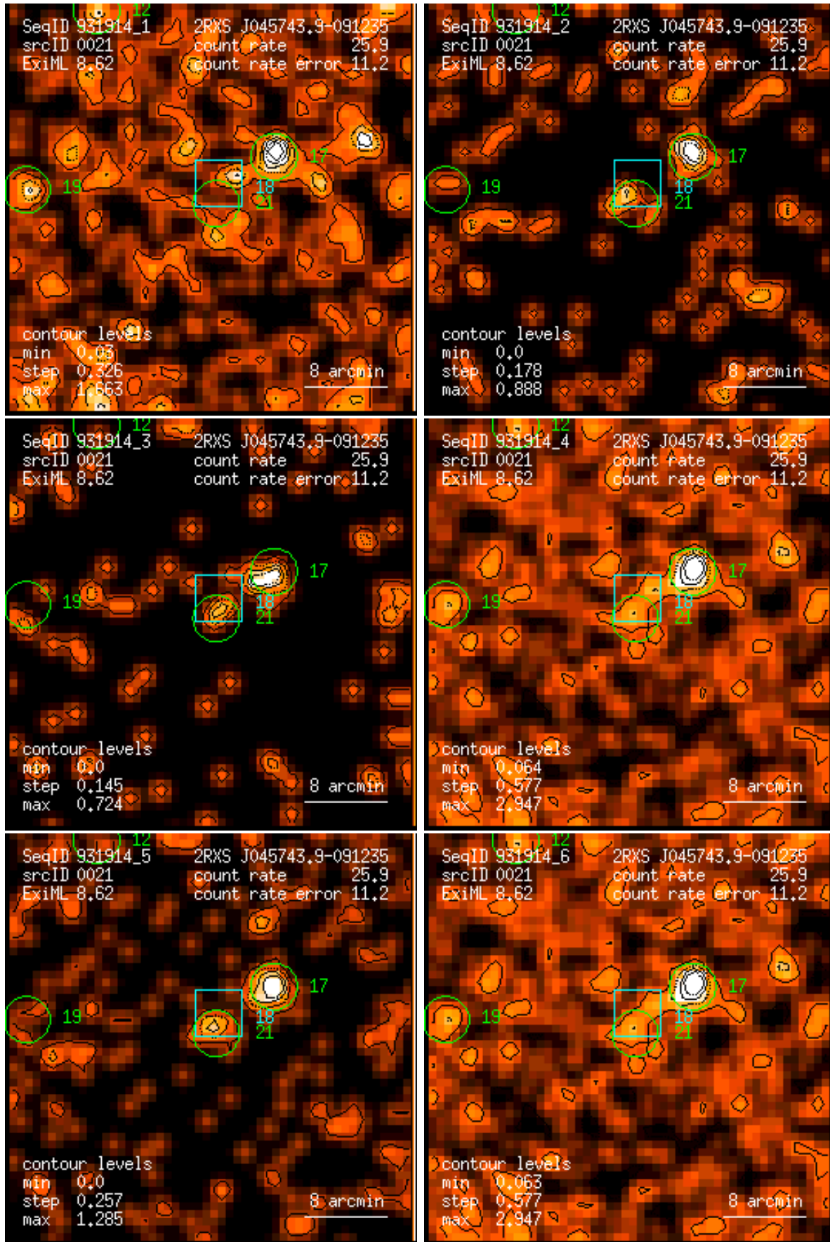
Figure 21: RASS 931914: detection 0021: band rate images, Gaussian filter: (1) PSPC channels 11 – 41, (2) 52 – 90, (3) 91 – 201, (4) 11 – 235, (5) 52 – 201, (6) 11 – 201. Broad band rates in counts/ks. Band rate contour levels in counts/ks/arcmin 2 .
