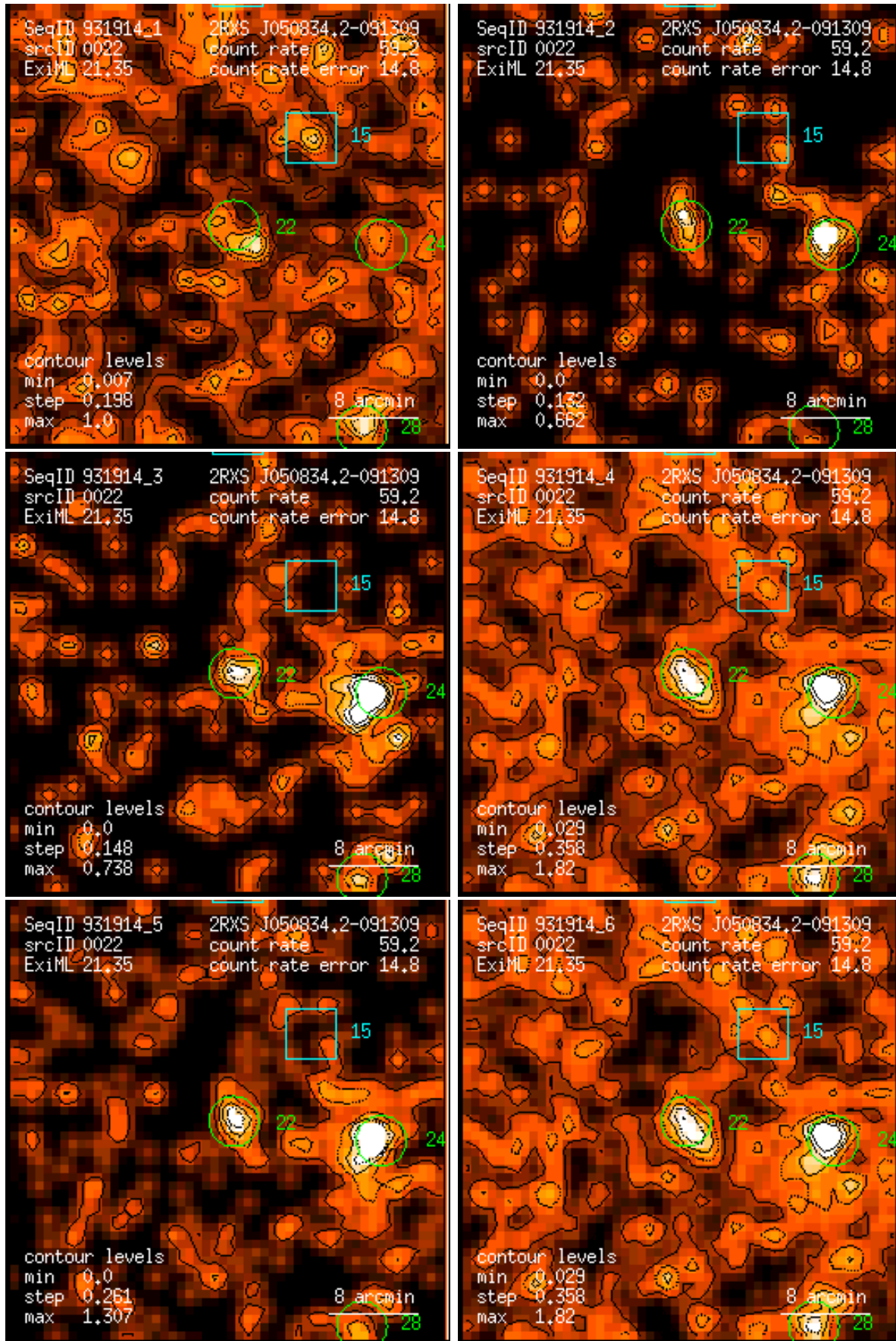
Figure 22: RASS 931914: detection 0022: band rate images, Gaussian filter: (1) PSPC channels 11 – 41, (2) 52 – 90, (3) 91 – 201, (4) 11 – 235, (5) 52 – 201, (6) 11 – 201. Broad band rates in counts/ks. Band rate contour levels in counts/ks/arcmin 2 .
