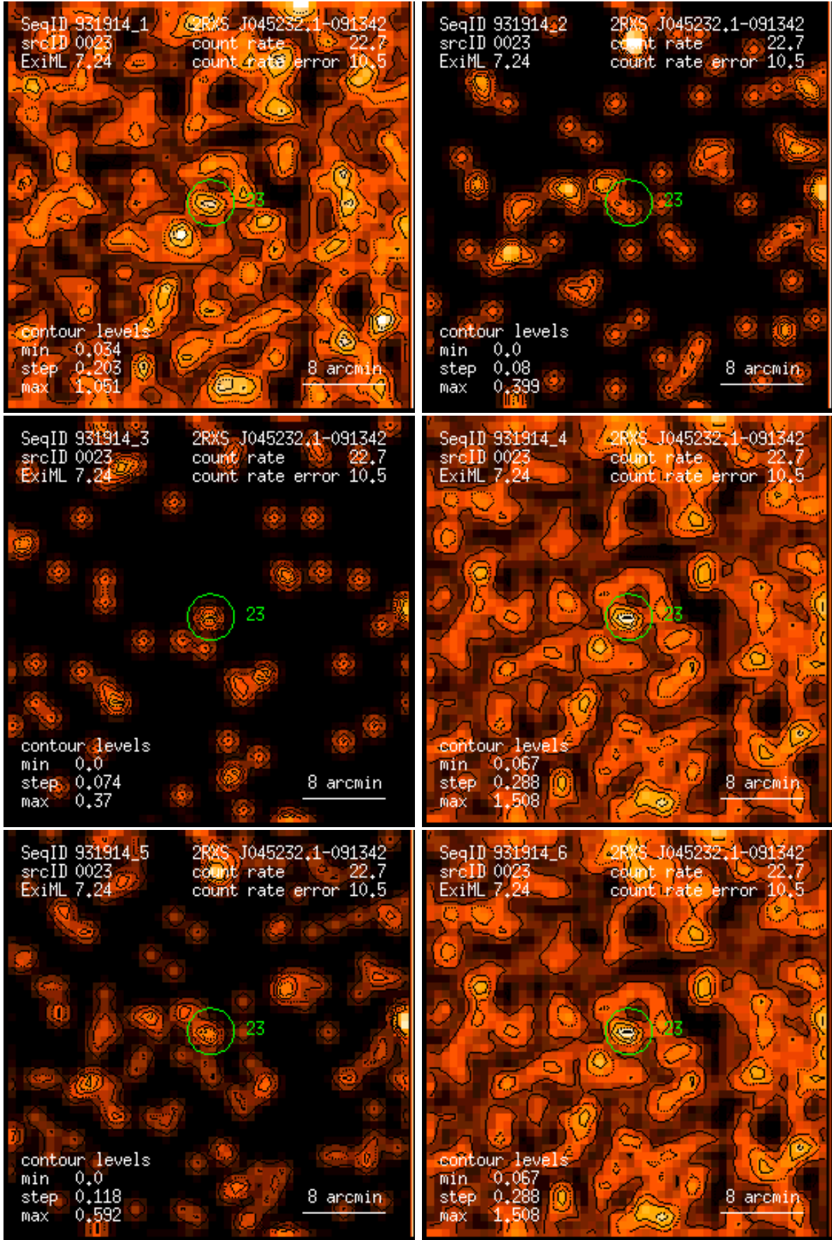
Figure 23: RASS 931914: detection 0023: band rate images, Gaussian filter: (1) PSPC channels 11 – 41, (2) 52 – 90, (3) 91 – 201, (4) 11 – 235, (5) 52 – 201, (6) 11 – 201. Broad band rates in counts/ks. Band rate contour levels in counts/ks/arcmin 2 .
