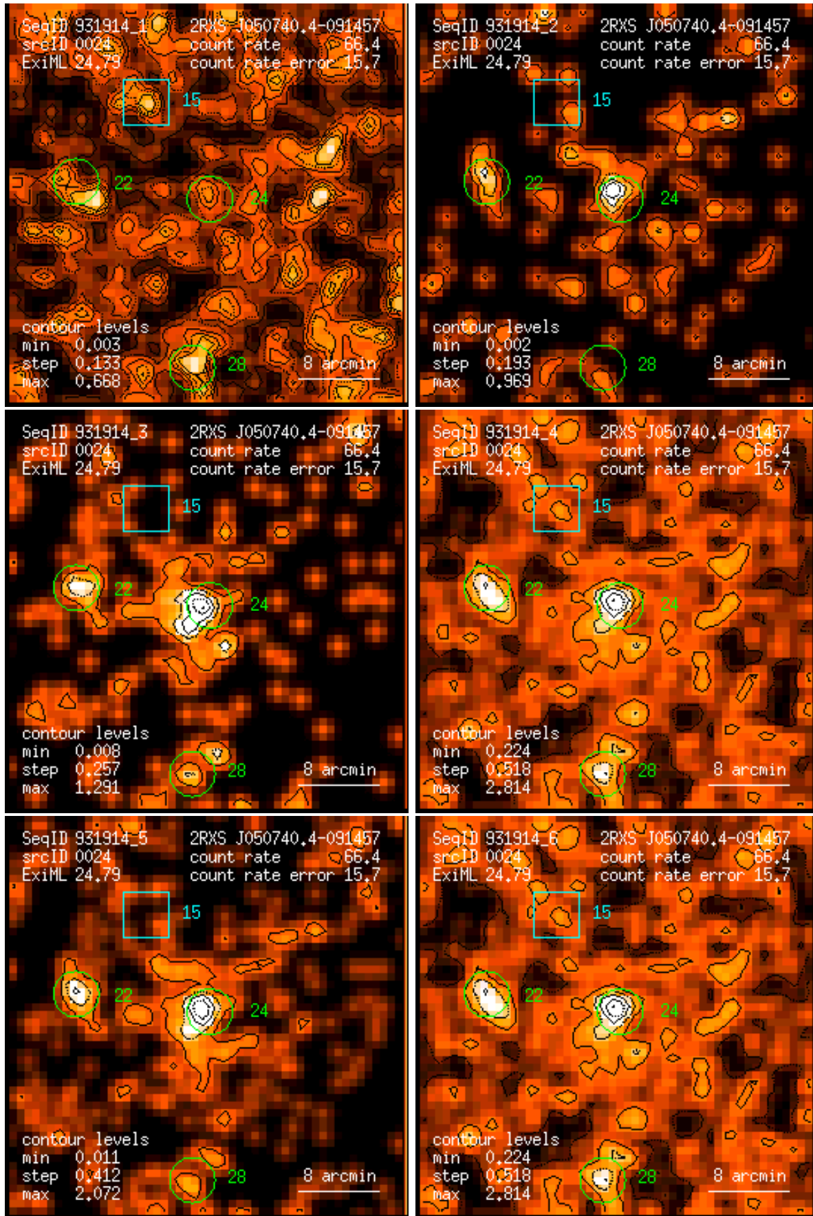
Figure 24: RASS 931914: detection 0024: band rate images, Gaussian filter: (1) PSPC channels 11 – 41, (2) 52 – 90, (3) 91 – 201, (4) 11 – 235, (5) 52 – 201, (6) 11 – 201. Broad band rates in counts/ks. Band rate contour levels in counts/ks/arcmin 2 .
