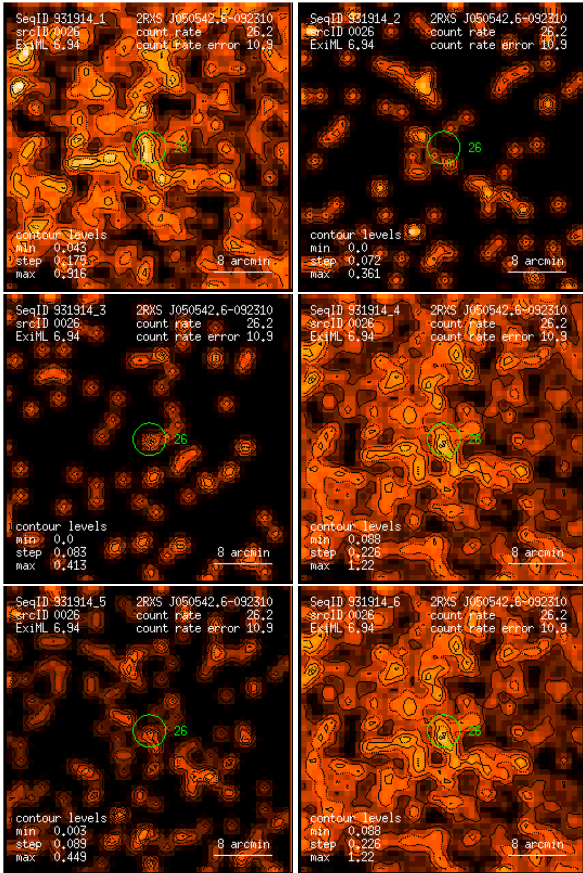
Figure 26: RASS 931914: detection 0026: band rate images, Gaussian filter: (1) PSPC channels 11 – 41, (2) 52 – 90, (3) 91 – 201, (4) 11 – 235, (5) 52 – 201, (6) 11 – 201. Broad band rates in counts/ks. Band rate contour levels in counts/ks/arcmin 2 .
