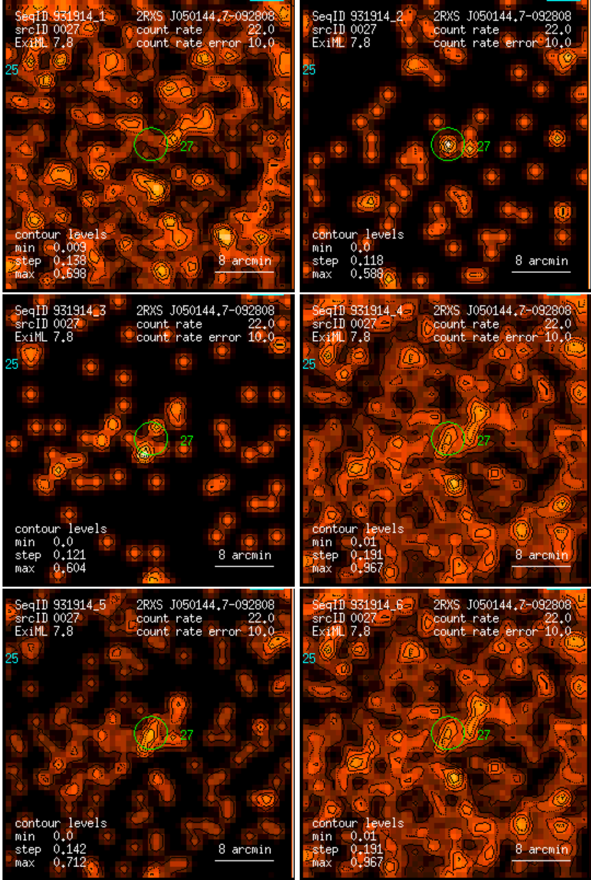
Figure 27: RASS 931914: detection 0027: band rate images, Gaussian filter: (1) PSPC channels 11 – 41, (2) 52 – 90, (3) 91 – 201, (4) 11 – 235, (5) 52 – 201, (6) 11 – 201. Broad band rates in counts/ks. Band rate contour levels in counts/ks/arcmin 2 .
