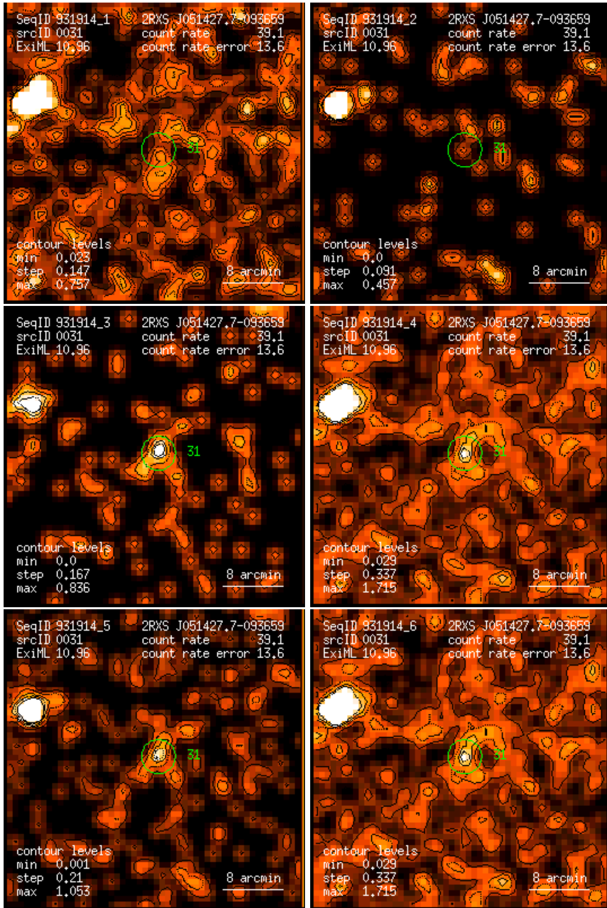
Figure 31: RASS 931914: detection 0031: band rate images, Gaussian filter: (1) PSPC channels 11 – 41, (2) 52 – 90, (3) 91 – 201, (4) 11 – 235, (5) 52 – 201, (6) 11 – 201. Broad band rates in counts/ks. Band rate contour levels in counts/ks/arcmin 2 .
