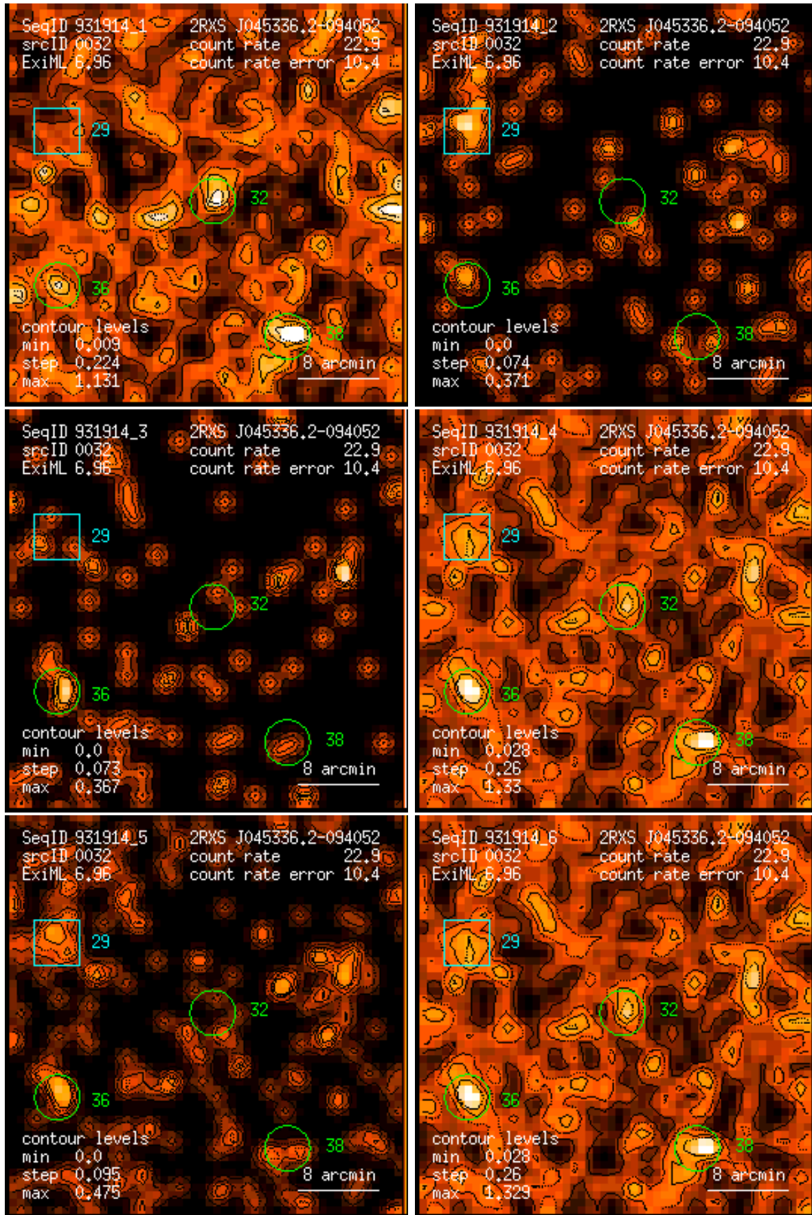
Figure 32: RASS 931914: detection 0032: band rate images, Gaussian filter: (1) PSPC channels 11 – 41, (2) 52 – 90, (3) 91 – 201, (4) 11 – 235, (5) 52 – 201, (6) 11 – 201. Broad band rates in counts/ks. Band rate contour levels in counts/ks/arcmin 2 .
