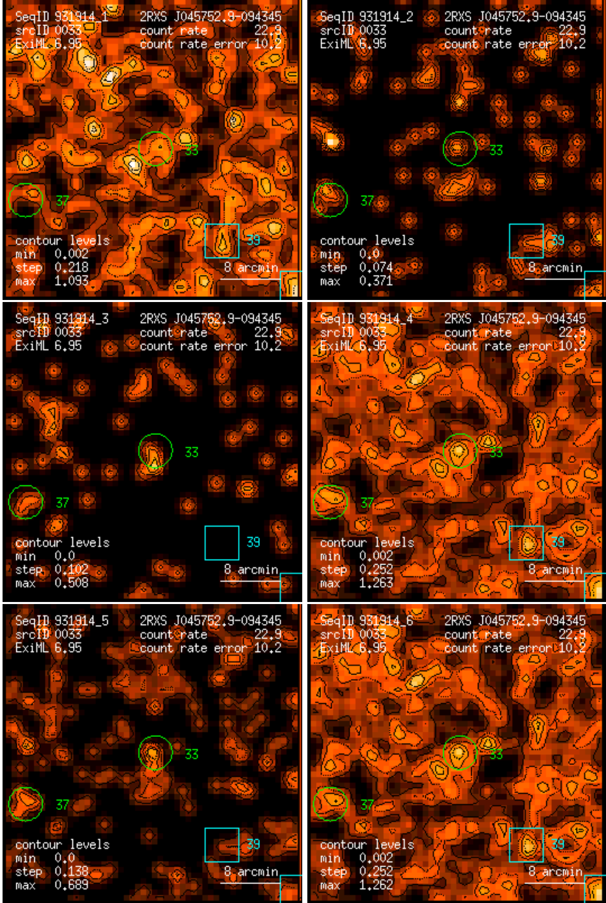
Figure 33: RASS 931914: detection 0033: band rate images, Gaussian filter: (1) PSPC channels 11 – 41, (2) 52 – 90, (3) 91 – 201, (4) 11 – 235, (5) 52 – 201, (6) 11 – 201. Broad band rates in counts/ks. Band rate contour levels in counts/ks/arcmin 2 .
