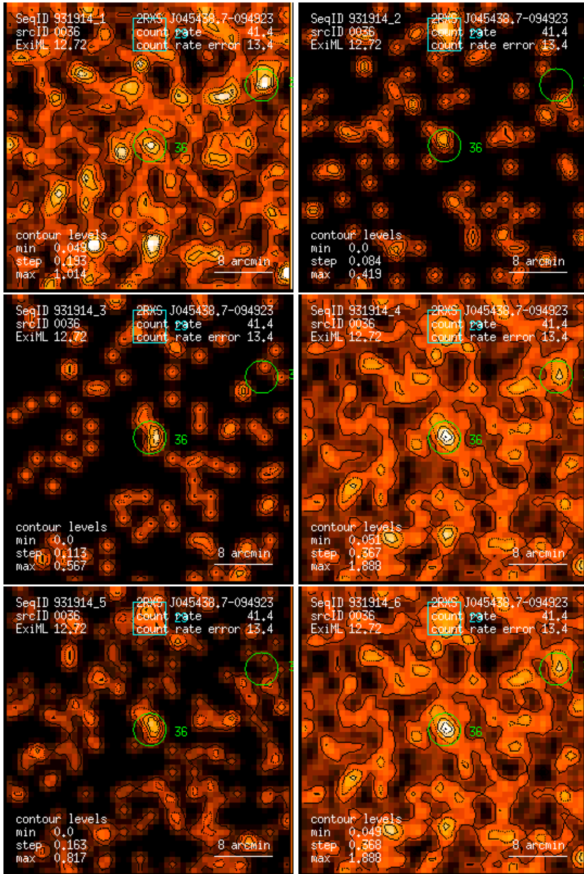
Figure 36: RASS 931914: detection 0036: band rate images, Gaussian filter: (1) PSPC channels 11 – 41, (2) 52 – 90, (3) 91 – 201, (4) 11 – 235, (5) 52 – 201, (6) 11 – 201. Broad band rates in counts/ks. Band rate contour levels in counts/ks/arcmin 2 .
