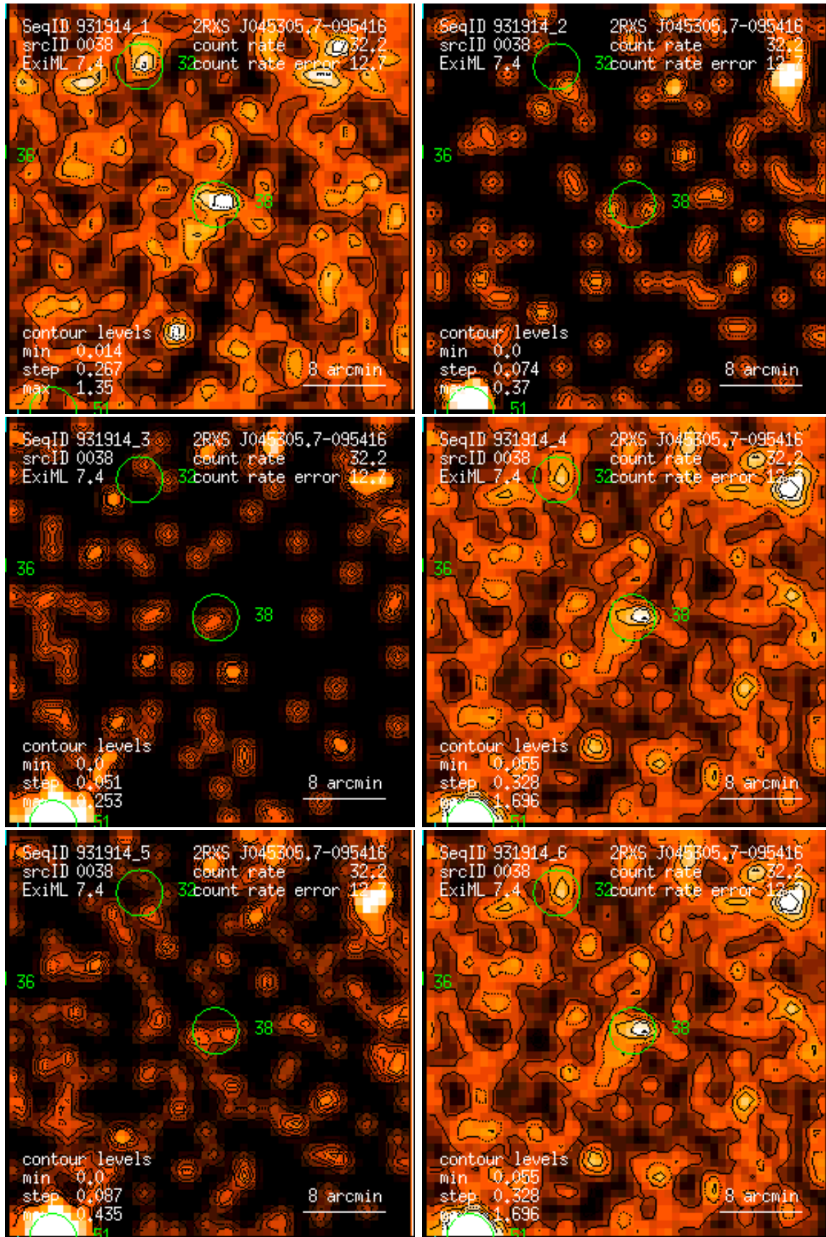
Figure 38: RASS 931914: detection 0038: band rate images, Gaussian filter: (1) PSPC channels 11 – 41, (2) 52 – 90, (3) 91 – 201, (4) 11 – 235, (5) 52 – 201, (6) 11 – 201. Broad band rates in counts/ks. Band rate contour levels in counts/ks/arcmin 2 .
