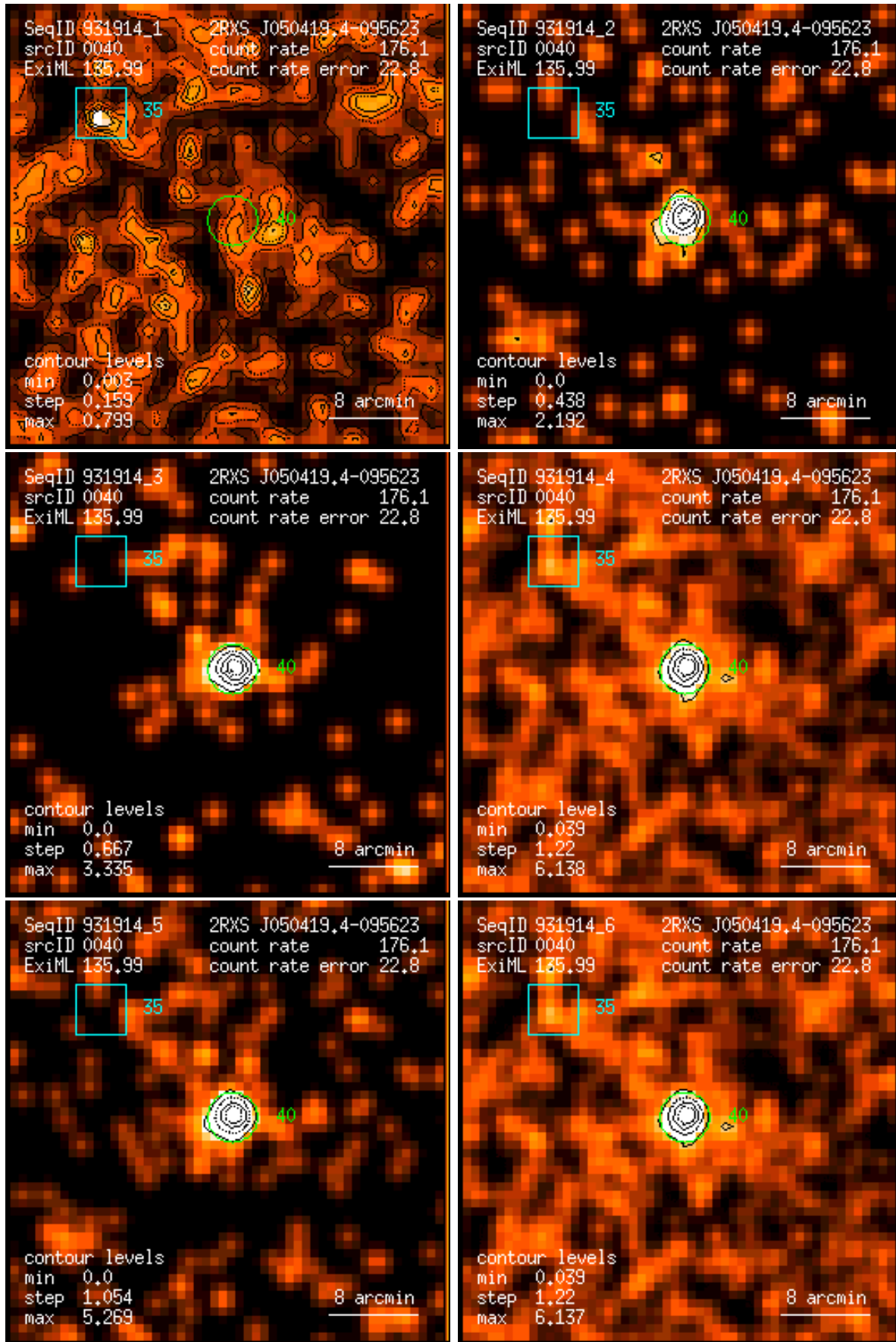
Figure 40: RASS 931914: detection 0040: band rate images, Gaussian filter: (1) PSPC channels 11 – 41, (2) 52 – 90, (3) 91 – 201, (4) 11 – 235, (5) 52 – 201, (6) 11 – 201. Broad band rates in counts/ks. Band rate contour levels in counts/ks/arcmin 2 .
