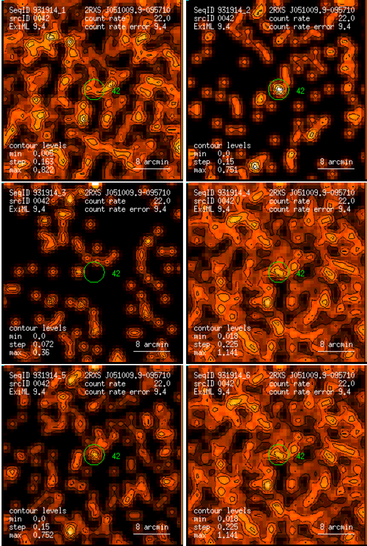
Figure 42: RASS 931914: detection 0042: band rate images, Gaussian filter: (1) PSPC channels 11 – 41, (2) 52 – 90, (3) 91 – 201, (4) 11 – 235, (5) 52 – 201, (6) 11 – 201. Broad band rates in counts/ks. Band rate contour levels in counts/ks/arcmin 2 .
