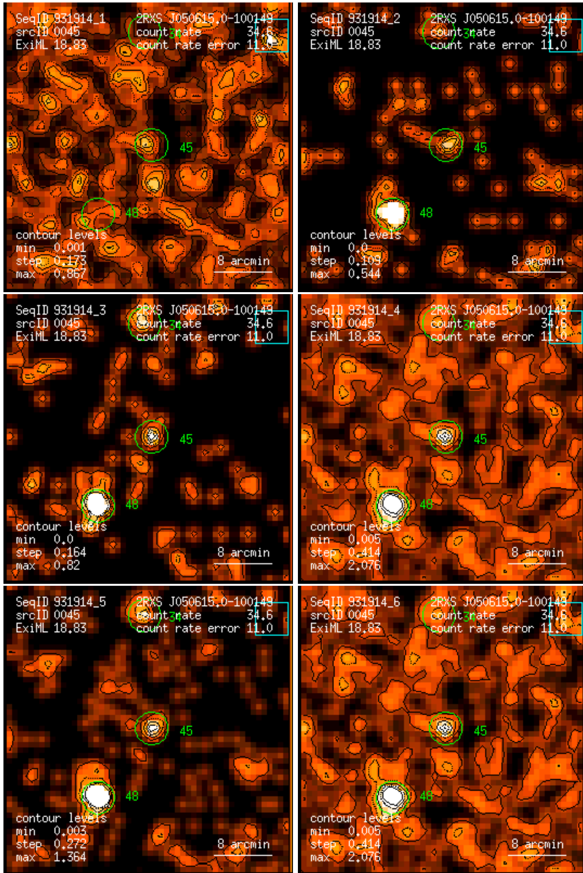
Figure 45: RASS 931914: detection 0045: band rate images, Gaussian filter: (1) PSPC channels 11 – 41, (2) 52 – 90, (3) 91 – 201, (4) 11 – 235, (5) 52 – 201, (6) 11 – 201. Broad band rates in counts/ks. Band rate contour levels in counts/ks/arcmin 2 .
