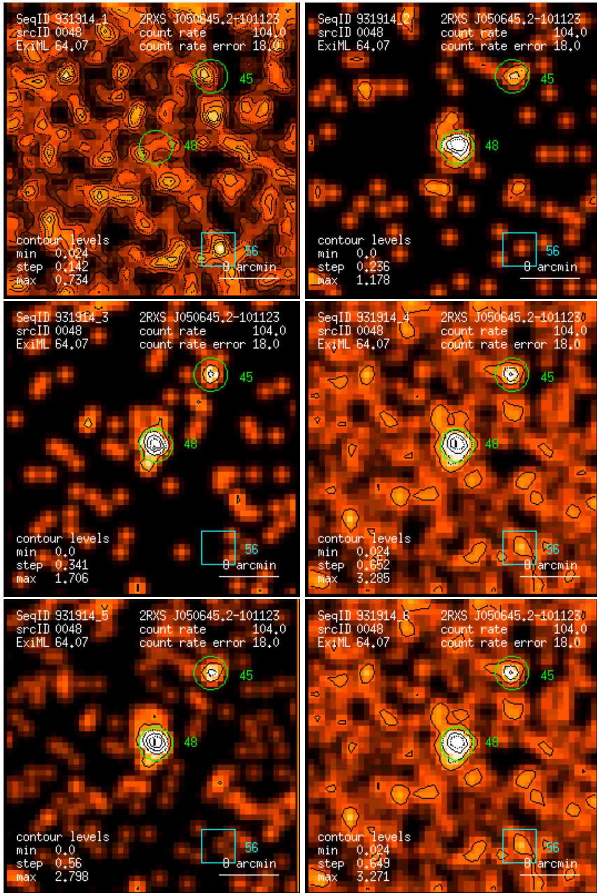
Figure 48: RASS 931914: detection 0048: band rate images, Gaussian filter: (1) PSPC channels 11 – 41, (2) 52 – 90, (3) 91 – 201, (4) 11 – 235, (5) 52 – 201, (6) 11 – 201. Broad band rates in counts/ks. Band rate contour levels in counts/ks/arcmin 2 .
