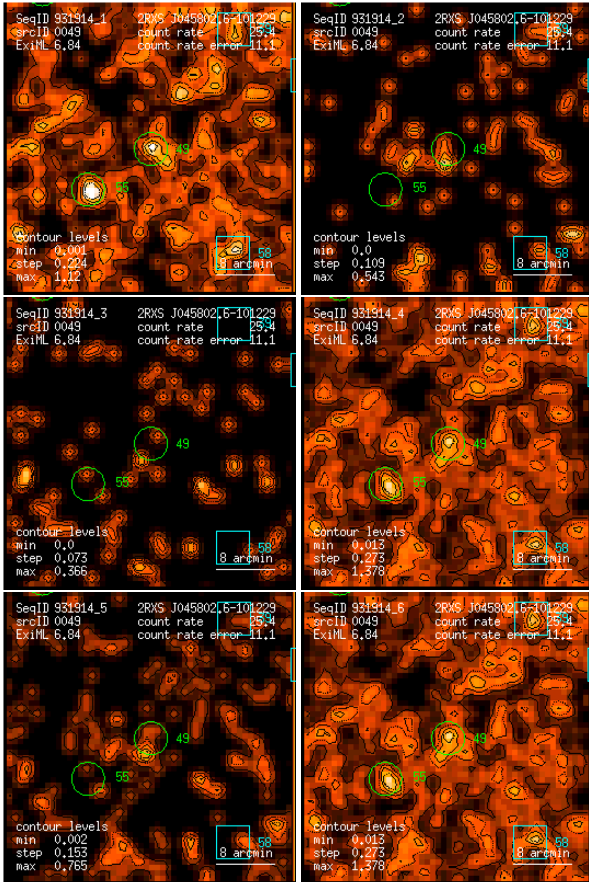
Figure 49: RASS 931914: detection 0049: band rate images, Gaussian filter: (1) PSPC channels 11 – 41, (2) 52 – 90, (3) 91 – 201, (4) 11 – 235, (5) 52 – 201, (6) 11 – 201. Broad band rates in counts/ks. Band rate contour levels in counts/ks/arcmin 2 .
