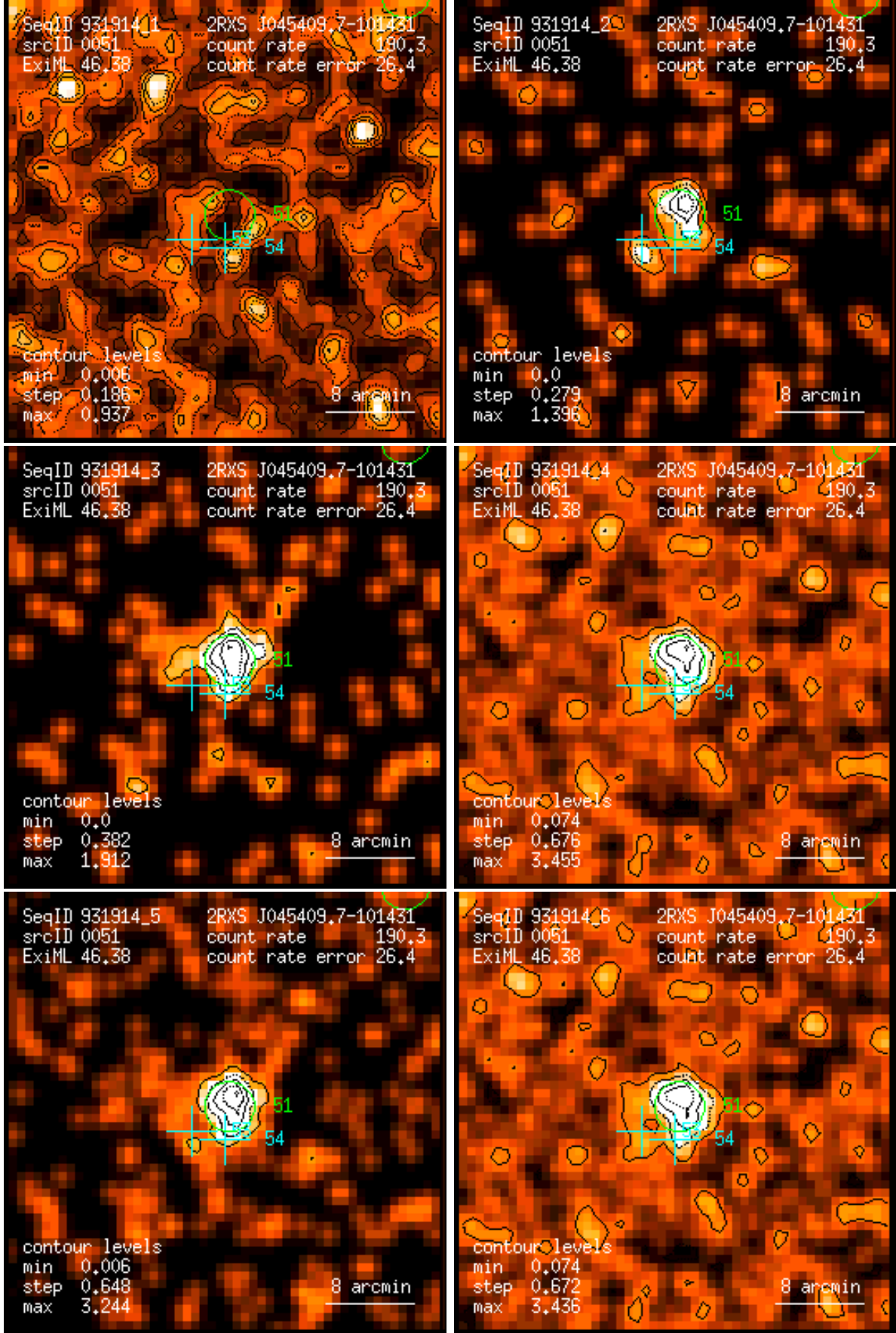
Figure 51: RASS 931914: detection 0051: band rate images, Gaussian filter: (1) PSPC channels 11 – 41, (2) 52 – 90, (3) 91 – 201, (4) 11 – 235, (5) 52 – 201, (6) 11 – 201. Broad band rates in counts/ks. Band rate contour levels in counts/ks/arcmin 2 .
