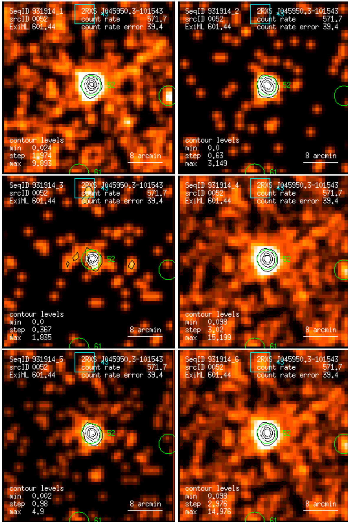
Figure 52: RASS 931914: detection 0052: band rate images, Gaussian filter: (1) PSPC channels 11 – 41, (2) 52 – 90, (3) 91 – 201, (4) 11 – 235, (5) 52 – 201, (6) 11 – 201. Broad band rates in counts/ks. Band rate contour levels in counts/ks/arcmin 2 .
