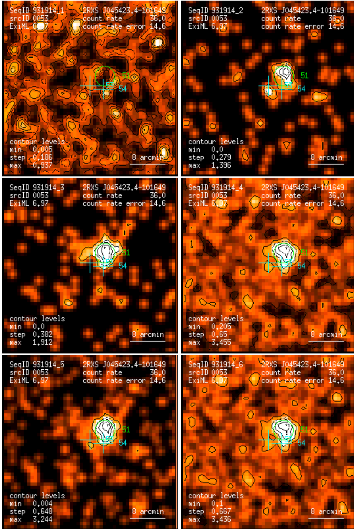
Figure 53: RASS 931914: detection 0053: band rate images, Gaussian filter: (1) PSPC channels 11 – 41, (2) 52 – 90, (3) 91 – 201, (4) 11 – 235, (5) 52 – 201, (6) 11 – 201. Broad band rates in counts/ks. Band rate contour levels in counts/ks/arcmin 2 .
