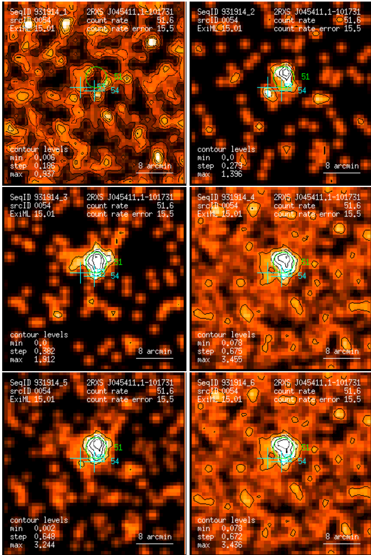
Figure 54: RASS 931914: detection 0054: band rate images, Gaussian filter: (1) PSPC channels 11 – 41, (2) 52 – 90, (3) 91 – 201, (4) 11 – 235, (5) 52 – 201, (6) 11 – 201. Broad band rates in counts/ks. Band rate contour levels in counts/ks/arcmin 2 .
