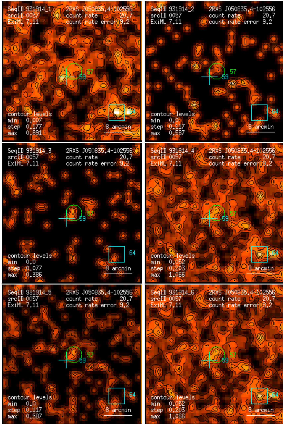
Figure 57: RASS 931914: detection 0057: band rate images, Gaussian filter: (1) PSPC channels 11 – 41, (2) 52 – 90, (3) 91 – 201, (4) 11 – 235, (5) 52 – 201, (6) 11 – 201. Broad band rates in counts/ks. Band rate contour levels in counts/ks/arcmin 2 .
