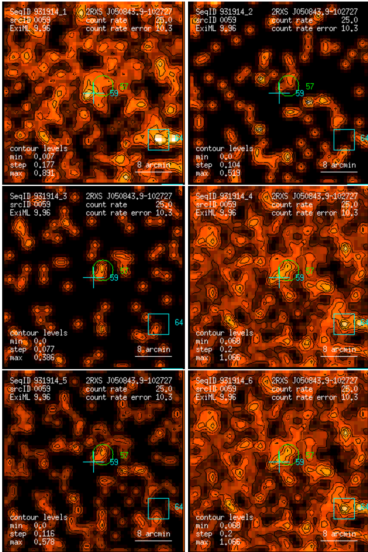
Figure 59: RASS 931914: detection 0059: band rate images, Gaussian filter: (1) PSPC channels 11 – 41, (2) 52 – 90, (3) 91 – 201, (4) 11 – 235, (5) 52 – 201, (6) 11 – 201. Broad band rates in counts/ks. Band rate contour levels in counts/ks/arcmin 2 .
