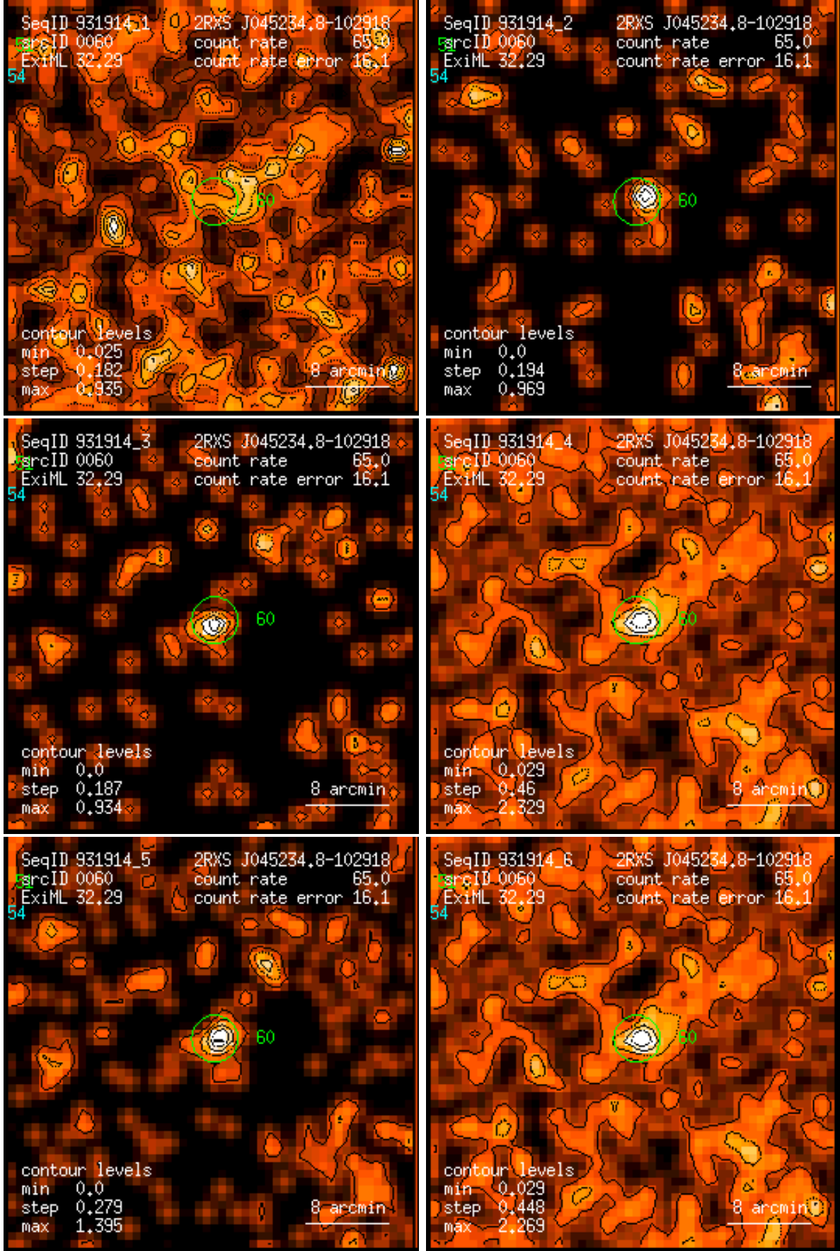
Figure 60: RASS 931914: detection 0060: band rate images, Gaussian filter: (1) PSPC channels 11 – 41, (2) 52 – 90, (3) 91 – 201, (4) 11 – 235, (5) 52 – 201, (6) 11 – 201. Broad band rates in counts/ks. Band rate contour levels in counts/ks/arcmin 2 .
