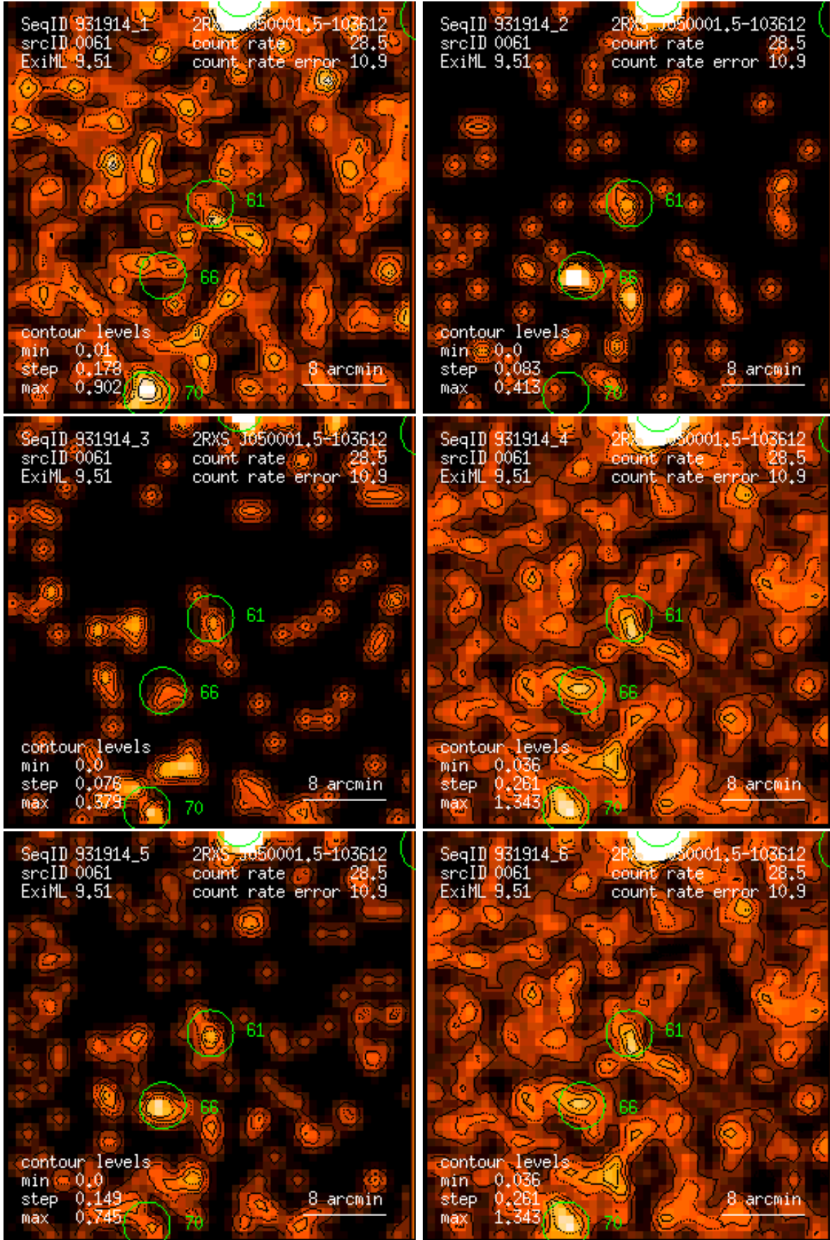
Figure 61: RASS 931914: detection 0061: band rate images, Gaussian filter: (1) PSPC channels 11 – 41, (2) 52 – 90, (3) 91 – 201, (4) 11 – 235, (5) 52 – 201, (6) 11 – 201. Broad band rates in counts/ks. Band rate contour levels in counts/ks/arcmin 2 .
