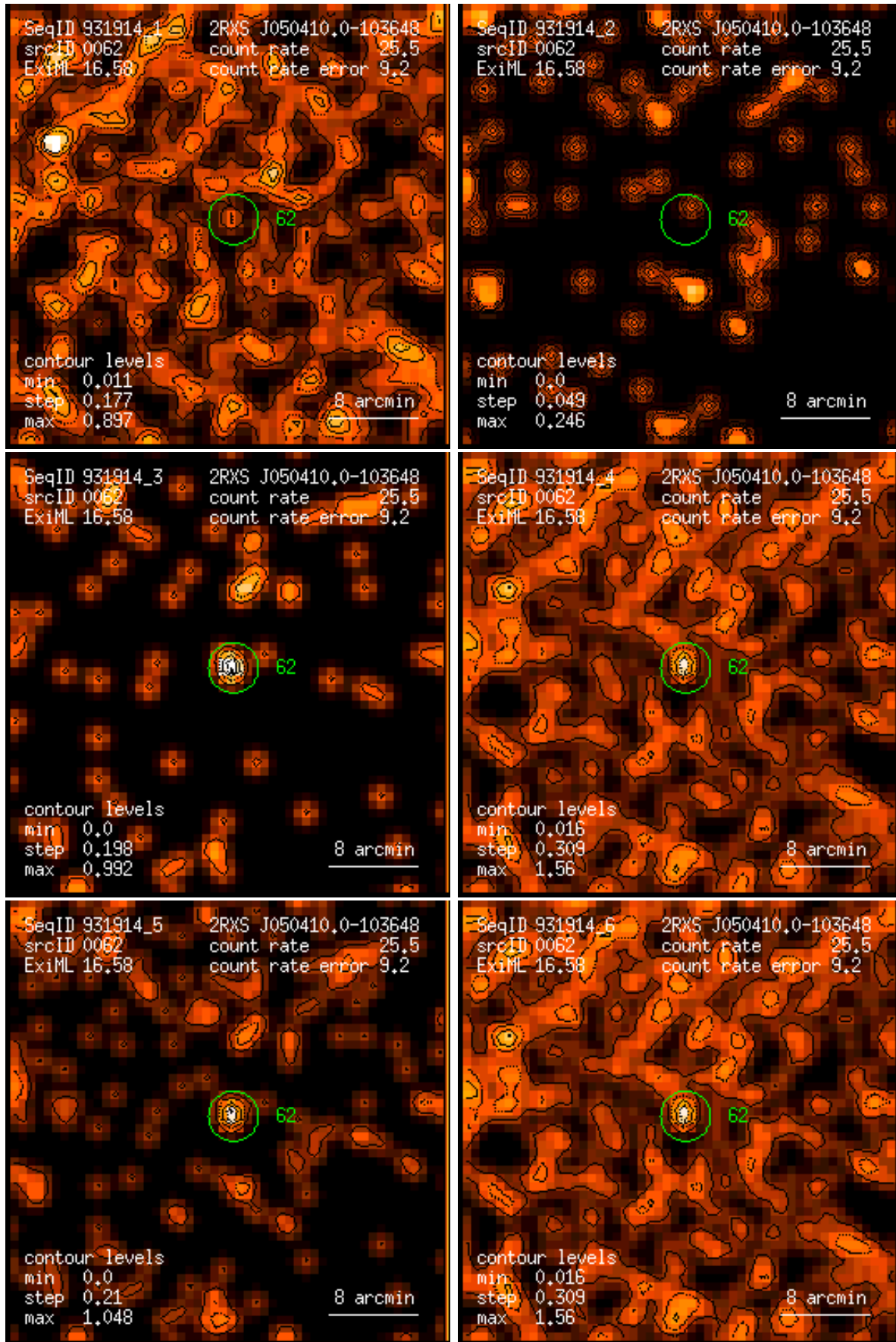
Figure 62: RASS 931914: detection 0062: band rate images, Gaussian filter: (1) PSPC channels 11 – 41, (2) 52 – 90, (3) 91 – 201, (4) 11 – 235, (5) 52 – 201, (6) 11 – 201. Broad band rates in counts/ks. Band rate contour levels in counts/ks/arcmin 2 .
