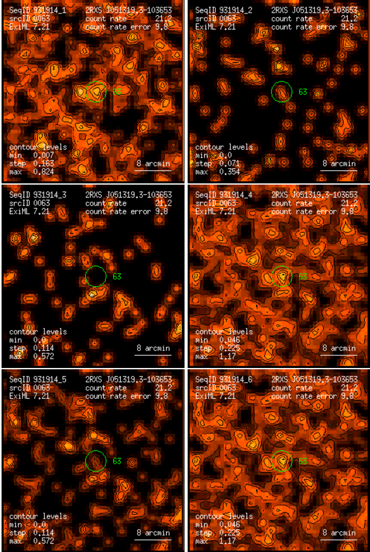
Figure 63: RASS 931914: detection 0063: band rate images, Gaussian filter: (1) PSPC channels 11 – 41, (2) 52 – 90, (3) 91 – 201, (4) 11 – 235, (5) 52 – 201, (6) 11 – 201. Broad band rates in counts/ks. Band rate contour levels in counts/ks/arcmin 2 .
