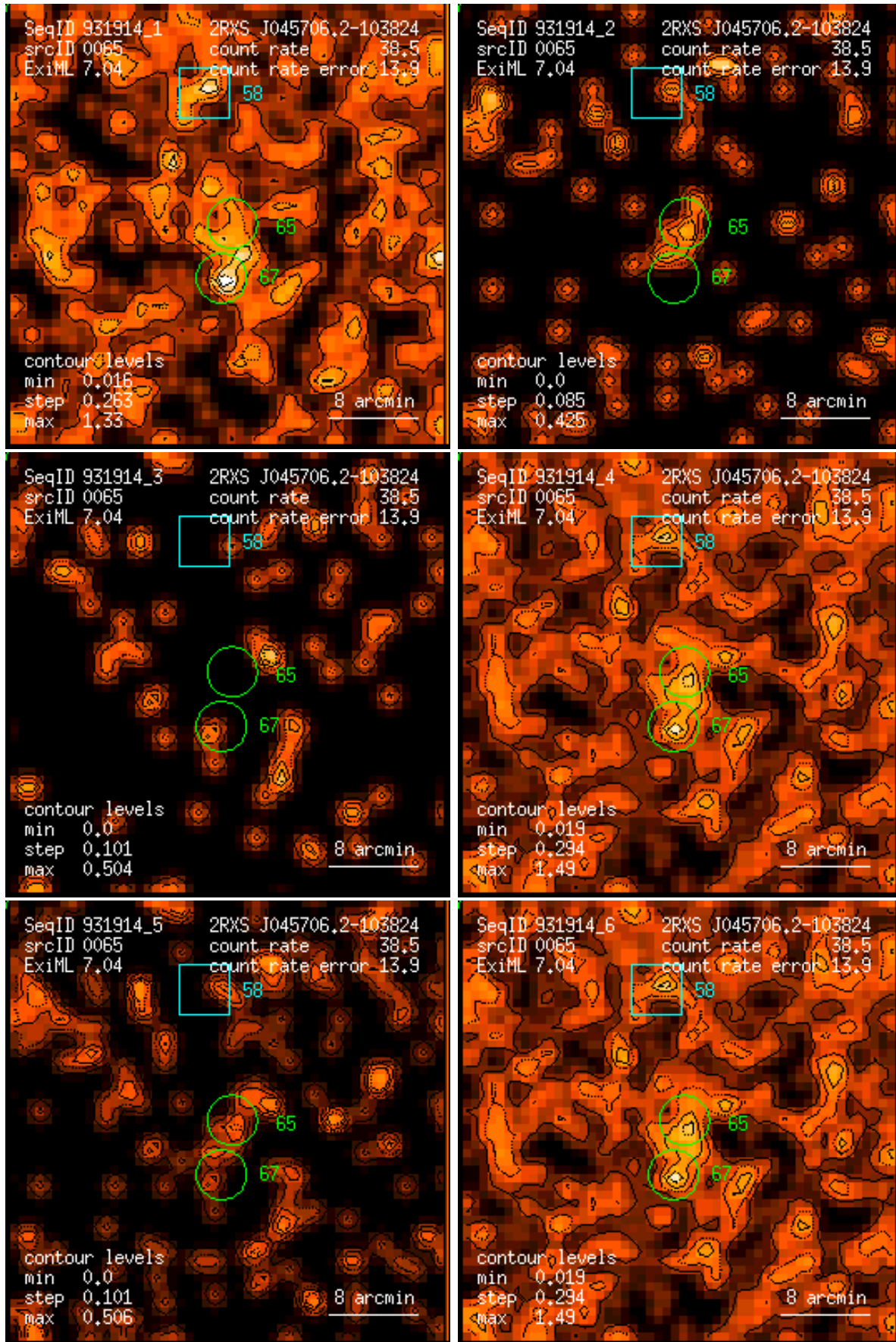
Figure 65: RASS 931914: detection 0065: band rate images, Gaussian filter: (1) PSPC channels 11 – 41, (2) 52 – 90, (3) 91 – 201, (4) 11 – 235, (5) 52 – 201, (6) 11 – 201. Broad band rates in counts/ks. Band rate contour levels in counts/ks/arcmin 2 .
