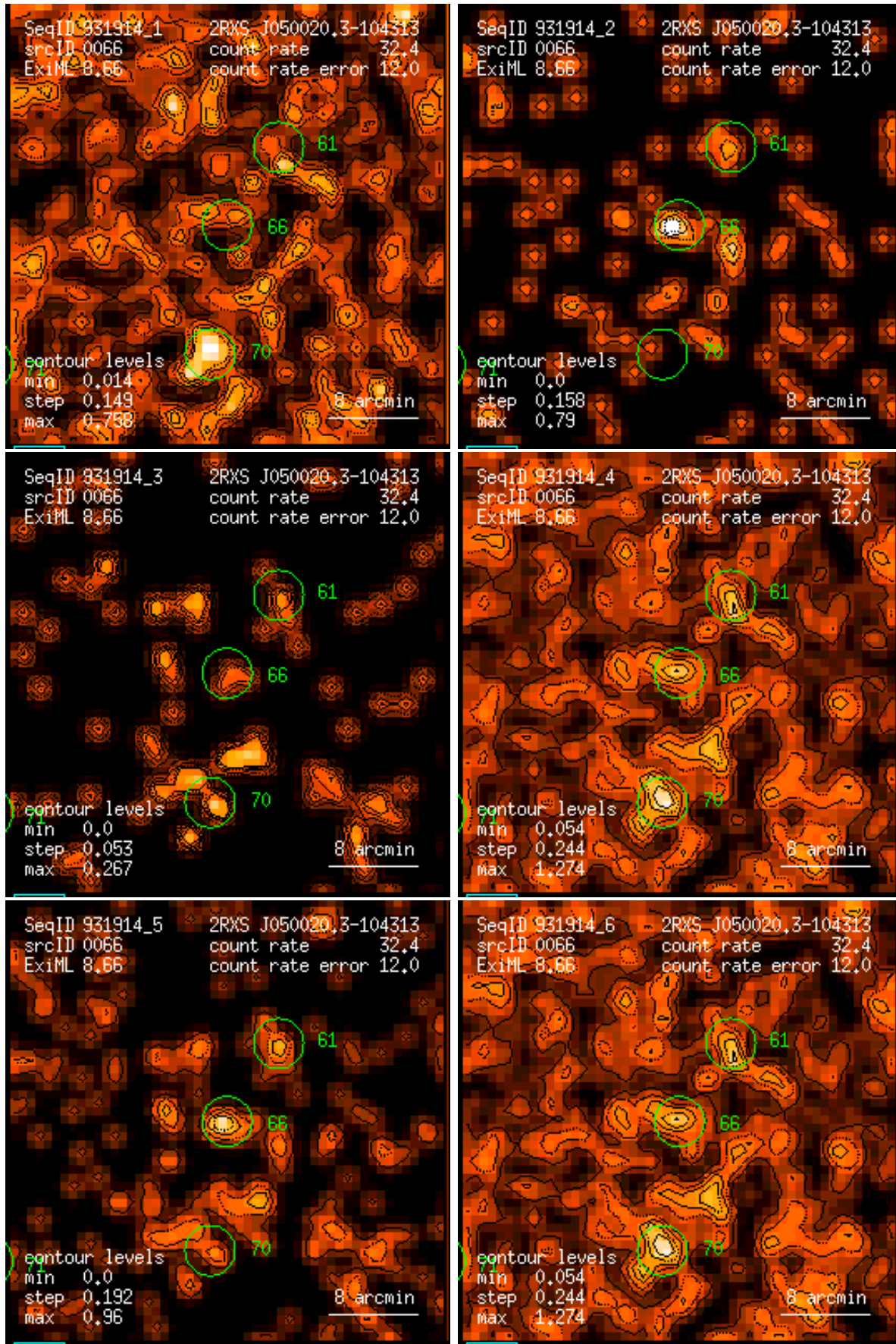
Figure 66: RASS 931914: detection 0066: band rate images, Gaussian filter: (1) PSPC channels 11 – 41, (2) 52 – 90, (3) 91 – 201, (4) 11 – 235, (5) 52 – 201, (6) 11 – 201. Broad band rates in counts/ks. Band rate contour levels in counts/ks/arcmin 2 .
