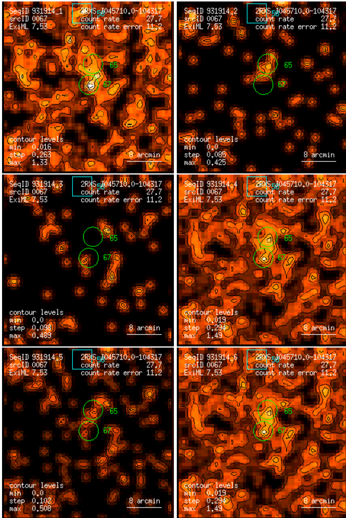
Figure 67: RASS 931914: detection 0067: band rate images, Gaussian filter: (1) PSPC channels 11 – 41, (2) 52 – 90, (3) 91 – 201, (4) 11 – 235, (5) 52 – 201, (6) 11 – 201. Broad band rates in counts/ks. Band rate contour levels in counts/ks/arcmin 2 .
